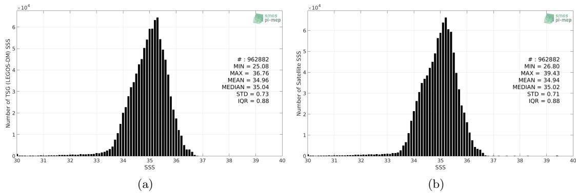
Figure 2: Histograms of SSS from TSG (LEGOS-DM) (a) and CCI SSS L4 Merged-OI v2.31 - 30-day running (ESA) (b) considering all match-up pairs per bins of 0.1 over the Tropical Pacific Ocean Pi-MEP region and for the full satellite product period.
