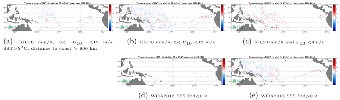
Figure 12: Temporal mean gridded over spatial boxes of size 1^{\circ}\times 1^{\circ} of \Delta\text{SSS} (CCI SSS L4 Merged-OI v2.31 - 30-day running (ESA) - TSG (LEGOS-DM)) for 5 different subdatasets corresponding to:RR=0 mm/h, 3 < U_{10} < 12 m/s, SST >5^{\circ}\text{C} , distance to coast > 800 km (a), RR=0 mm/h, 3 < U_{10} < 12 m/s (b), RR >1 mm/h and U_{10} < 4 m/s (c), WOA2013 SSS Std <0.2 (d), WOA2013 SSS Std >0.2 (e).
