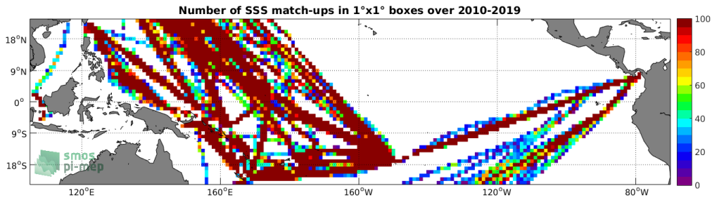
Figure 4: Number of SSS match-ups between TSG (LEGOS-DM) SSS and the CCI SSS L4 Merged-OI v2.31 - 30-day running (ESA) SSS product for the Tropical Pacific Ocean Pi-MEP region over 1°x1° boxes and for the full satellite product period.
