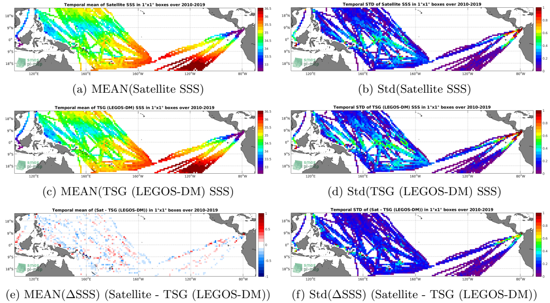
Figure 6: Temporal mean (left) and Std (right) of SSS from CCI SSS L4 Merged-OI v2.31 - 30-day running (ESA) (top), TSG (LEGOS-DM) (middle), and of \Delta SSS (Satellite - TSG (LEGOS-DM)). Only match-up pairs are used to generate these maps.
