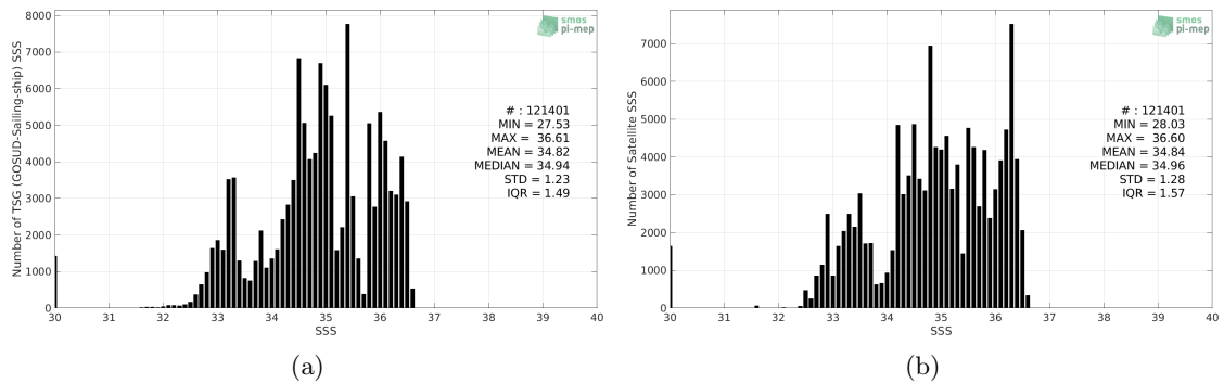
Figure 2: Histograms of SSS from TSG (GOSUD-Sailing-ship) (a) and CCI SSS L4 Merged-OI v2.31 - 30-day running (ESA) (b) considering all match-up pairs per bins of 0.1 over the Tropical Pacific Ocean Pi-MEP region and for the full satellite product period.
