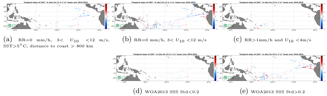
Figure 12: Temporal mean gridded over spatial boxes of size 1^{\circ}\times 1^{\circ} of \Delta SSS (CCI SSS L4 Merged-OI v2.31 - 30-day running (ESA) - TSG (GOSUD-Research-vessel)) for 5 different subdatasets corresponding to:RR=0 mm/h, 3 < U_{10} < 12 m/s, SST >5^{\circ}\text{C} , distance to coast > 800 km (a), RR=0 mm/h, 3 < U_{10} < 12 m/s (b), RR >1 mm/h and U_{10} < 4 m/s (c), WOA2013 SSS Std <0.2 (d), WOA2013 SSS Std >0.2 (e).
