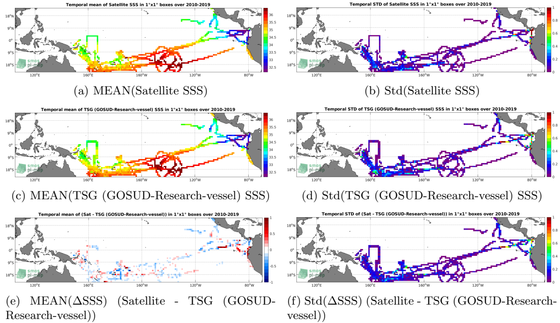
Figure 6: Temporal mean (left) and Std (right) of SSS from CCI SSS L4 Merged-OI v2.31 - 30-day running (ESA) (top), TSG (GOSUD-Research-vessel) (middle), and of \Delta SSS (Satellite - TSG (GOSUD-Research-vessel)). Only match-up pairs are used to generate these maps.
