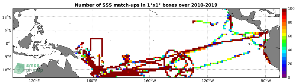
Figure 4: Number of SSS match-ups between TSG (GOSUD-Research-vessel) SSS and the CCI SSS L4 Merged-OI v2.31 - 30-day running (ESA) SSS product for the Tropical Pacific Ocean Pi-MEP region over 1°x1° boxes and for the full satellite product period.
