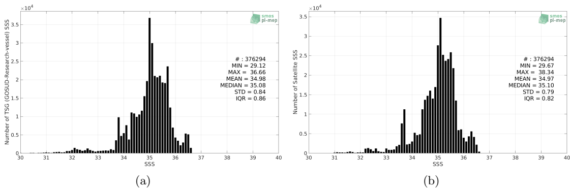
Figure 2: Histograms of SSS from TSG (GOSUD-Research-vessel) (a) and CCI SSS L4 Merged-OI v2.31 - 30-day running (ESA) (b) considering all match-up pairs per bins of 0.1 over the Tropical Pacific Ocean Pi-MEP region and for the full satellite product period.
