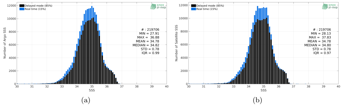
Figure 2: Histograms of SSS from Argo (a) and CCI SSS L4 Merged-OI v2.31 - 30-day running (ESA) (b) considering all match-up pairs per bins of 0.1 over the Tropical Pacific Ocean Pi-MEP region and for the full satellite product period.
