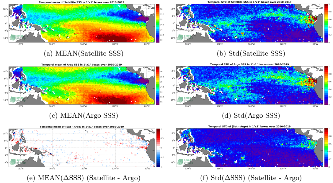
Figure 6: Temporal mean (left) and Std (right) of SSS from CCI SSS L4 Merged-OI v2.31 - 30-day running (ESA) (top), Argo (middle), and of \Delta SSS (Satellite - Argo). Only match-up pairs are used to generate these maps.
