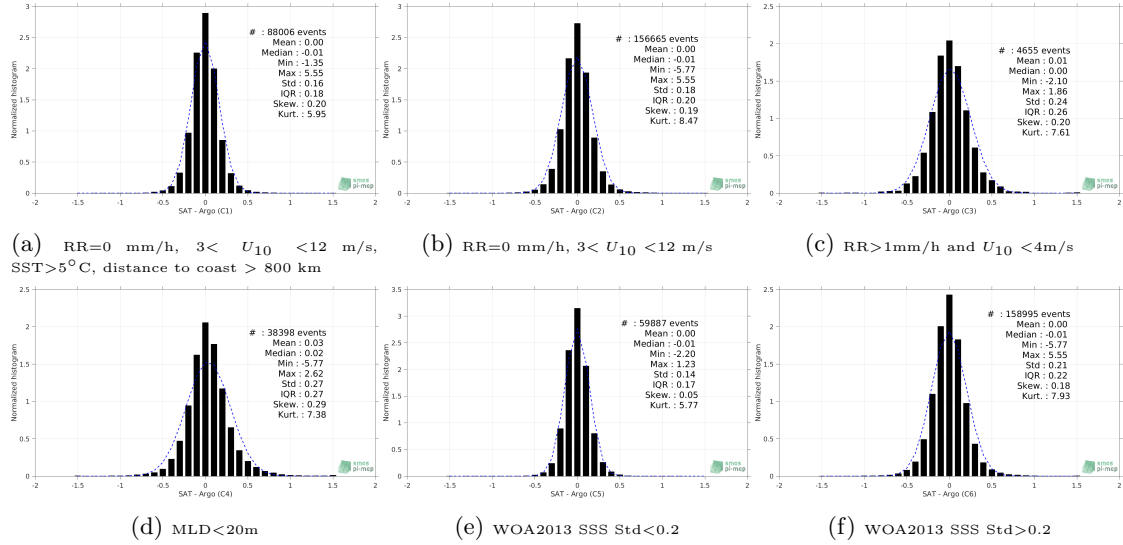
Figure 13: Normalized histogram of \Delta SSS (CCI SSS L4 Merged-OI v2.31 - 30-day running (ESA) - Argo) for 6 different subdatasets corresponding to: RR=0 mm/h, 3 < U_{10} < 12 m/s, SST >5^{\circ} C, distance to coast > 800 km (a), RR=0 mm/h, 3 < U_{10} < 12 m/s (b), RR >1 mm/h and U_{10} < 4 m/s (c), MLD <20 m (d), WOA2013 SSS Std <0.2 (e), WOA2013 SSS Std >0.2 (f).
