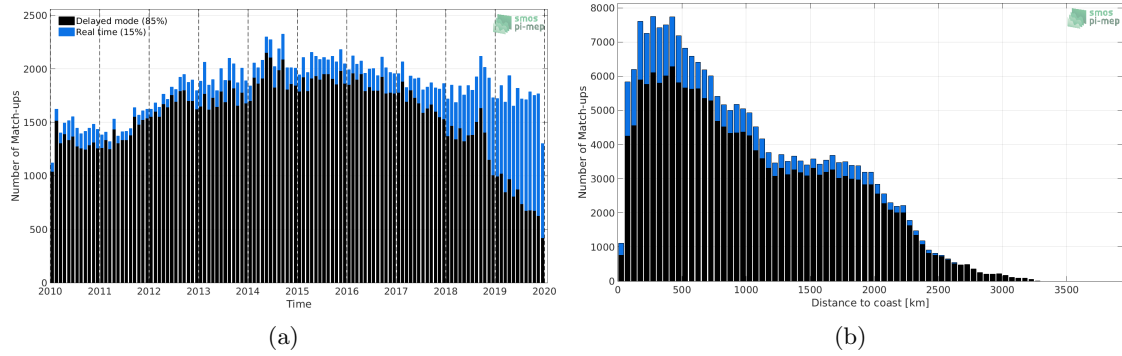
Figure 1: Number of match-ups between Argo and CCI SSS L4 Merged-OI v2.31 - 30-day running (ESA) SSS as a function of time (a) and as function of the distance to coast (b) over the Tropical Pacific Ocean Pi-MEP region and for the full satellite product period.
