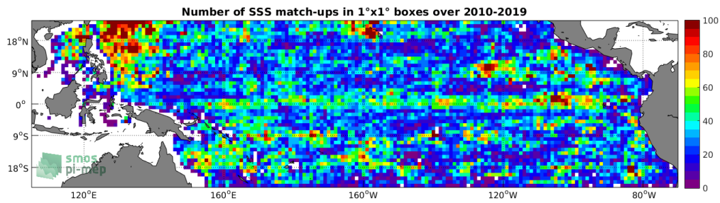
Figure 4: Number of SSS match-ups between Argo SSS and the CCI SSS L4 Merged-OI v2.31 - 30-day running (ESA) SSS product for the Tropical Pacific Ocean Pi-MEP region over 1^\circ \times 1^\circ boxes and for the full satellite product period.
