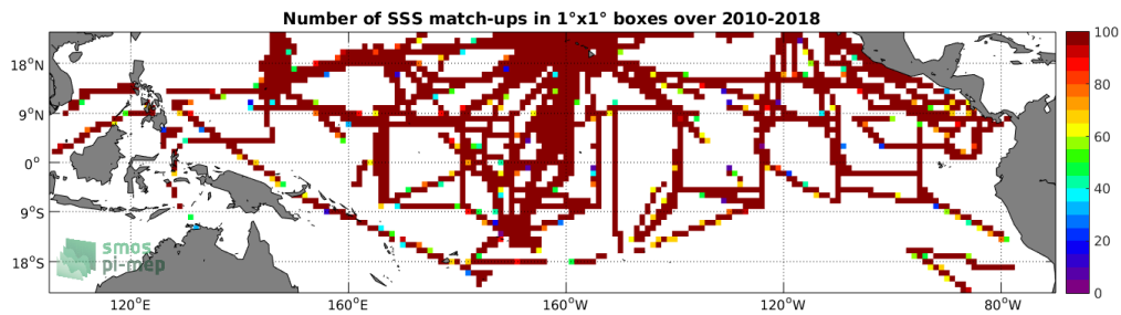
Figure 4: Number of SSS match-ups between TSG-SAMOS SSS and the CCI L4 Merged-OI v1.8 - 7-day running (ESA) SSS product for the Tropical Pacific Ocean Pi-MEP region over 1^\circ \times 1^\circ boxes and for the full satellite product period.
