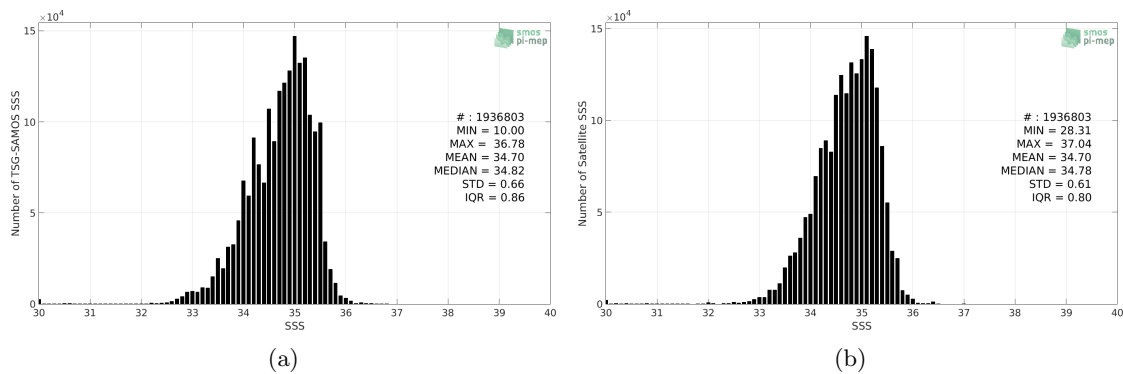
Figure 2: Histograms of SSS from TSG-SAMOS (a) and CCI L4 Merged-OI v1.8 - 7-day running (ESA) (b) considering all match-up pairs per bins of 0.1 over the Tropical Pacific Ocean Pi-MEP region and for the full satellite product period.
