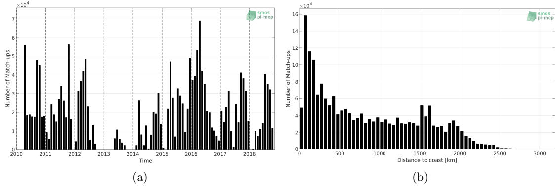
Figure 1: Number of match-ups between TSG-SAMOS and CCI L4 Merged-OI v1.8 - 7-day running (ESA) SSS as a function of time (a) and as function of the distance to coast (b) over the Tropical Pacific Ocean Pi-MEP region and for the full satellite product period.
