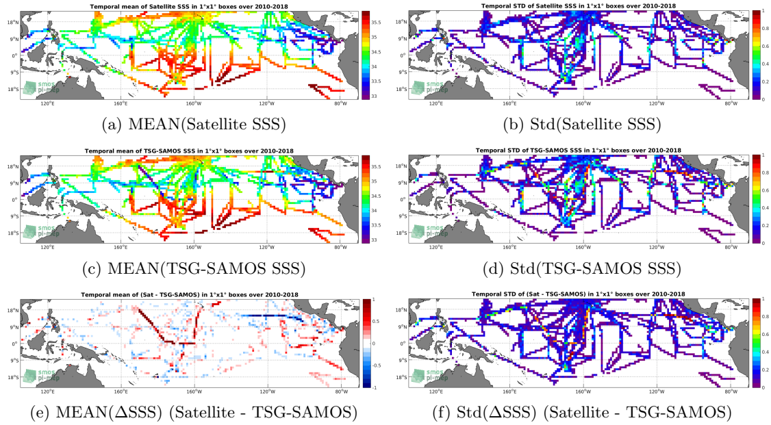
Figure 6: Temporal mean (left) and Std (right) of SSS from CCI L4 Merged-OI v1.8 - 7-day running (ESA) (top), TSG-SAMOS (middle), and of \Delta SSS (Satellite - TSG-SAMOS). Only match-up pairs are used to generate these maps.
