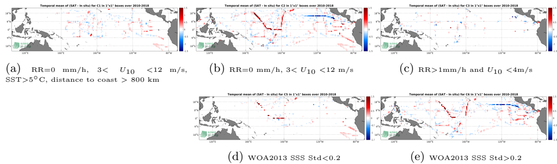
Figure 12: Temporal mean gridded over spatial boxes of size 1^\circ \times 1^\circ of \Delta SSS (CCI L4 Merged-OI v1.8 - 7-day running (ESA) - TSG-SAMOS) for 5 different subdatasets corresponding to:RR=0 mm/h, 3 < U_{10} < 12 m/s, SST > 5^\circ\text{C} , distance to coast > 800 km (a), RR=0 mm/h, 3 < U_{10} < 12 m/s (b), RR > 1 mm/h and U_{10} < 4 m/s (c), WOA2013 SSS Std < 0.2 (d), WOA2013 SSS Std > 0.2 (e).
