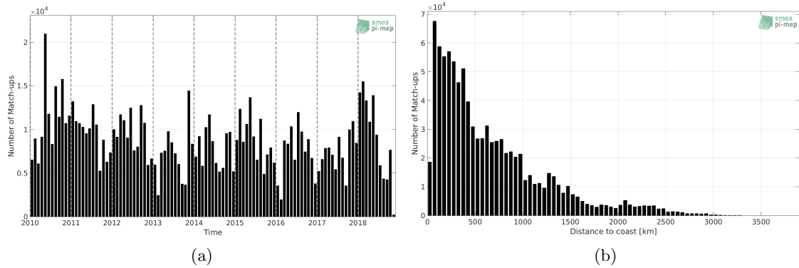
Figure 1: Number of match-ups between TSG-LEGOS-DM and CCI-L4-ESA-MERGED-OI-V1.8-7DAY-RUNNING SSS as a function of time (a) and as function of the distance to coast (b) over the Tropical Pacific Ocean Pi-MEP region and for the full satellite product period.
