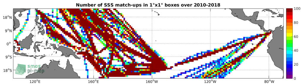
Figure 4: Number of SSS match-ups between TSG-LEGOS-DM SSS and the CCI-L4-ESA-MERGED-OI-V1.8-7DAY-RUNNING SSS product for the Tropical Pacific Ocean Pi-MEP region over 1^\circ \times 1^\circ boxes and for the full satellite product period.
