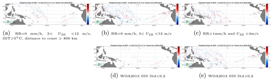
Figure 12: Temporal mean gridded over spatial boxes of size 1^\circ \times 1^\circ of \Delta SSS (CCI-L4-ESAMERGED-OI-V1.8-7DAY-RUNNING - TSG-LEGOS-DM) for 5 different subdatasets corresponding to:RR=0 mm/h, 3 < U_{10} < 12 m/s, SST >5^\circ C, distance to coast > 800 km (a), RR=0 mm/h, 3 < U_{10} < 12 m/s (b), RR >1 mm/h and U_{10} < 4 m/s (c), WOA2013 SSS Std <0.2 (d), WOA2013 SSS Std >0.2 (e).
