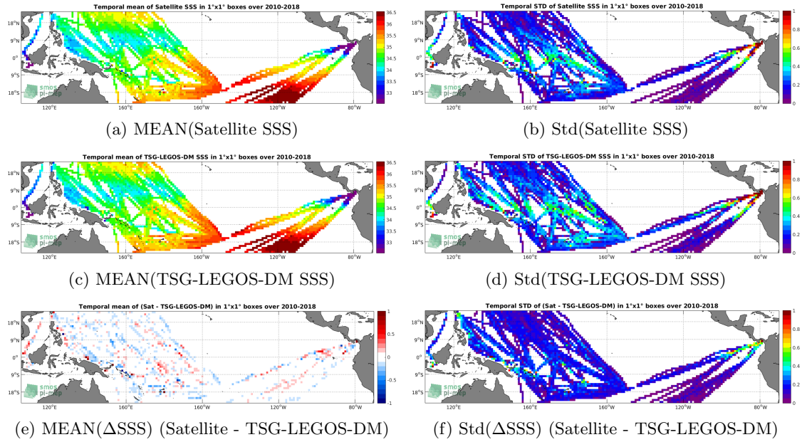
Figure 6: Temporal mean (left) and Std (right) of SSS from CCI-L4-ESA-MERGED-OI-V1.8-7DAY-RUNNING (top), TSG-LEGOS-DM (middle), and of \Delta SSS (Satellite - TSG-LEGOS-DM). Only match-up pairs are used to generate these maps.
