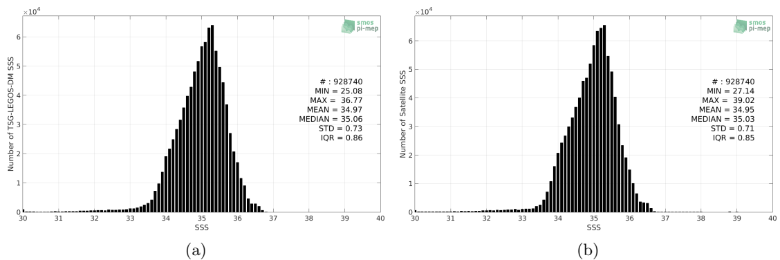
Figure 2: Histograms of SSS from TSG-LEGOS-DM (a) and CCI-L4-ESA-MERGED-OI-V1.8-7DAY-RUNNING (b) considering all match-up pairs per bins of 0.1 over the Tropical Pacific Ocean Pi-MEP region and for the full satellite product period.
