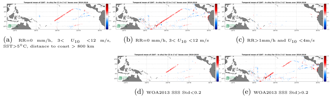
Figure 12: Temporal mean gridded over spatial boxes of size 1^{\circ}\times 1^{\circ} of \Delta SSS (CCI L4 Merged-OI v1.8 - 7-day running (ESA) - TSG-GOSUD-Research-vessel) for 5 different subdatasets corresponding to:RR=0 mm/h, 3 < U_{10} < 12 m/s, SST >5^{\circ}\text{C} , distance to coast > 800 km (a), RR=0 mm/h, 3 < U_{10} < 12 m/s (b), RR >1 mm/h and U_{10} < 4 m/s (c), WOA2013 SSS Std <0.2 (d), WOA2013 SSS Std >0.2 (e).
