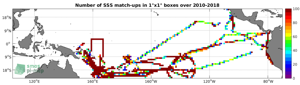
Figure 4: Number of SSS match-ups between TSG-GOSUD-Research-vessel SSS and the CCI L4 Merged-OI v1.8 - 7-day running (ESA) SSS product for the Tropical Pacific Ocean Pi-MEP region over 1^\circ \times 1^\circ boxes and for the full satellite product period.
