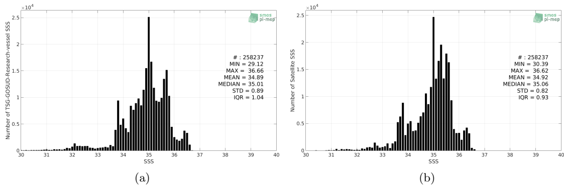
Figure 2: Histograms of SSS from TSG-GOSUD-Research-vessel (a) and CCI L4 Merged-OI v1.8 - 7-day running (ESA) (b) considering all match-up pairs per bins of 0.1 over the Tropical Pacific Ocean Pi-MEP region and for the full satellite product period.
