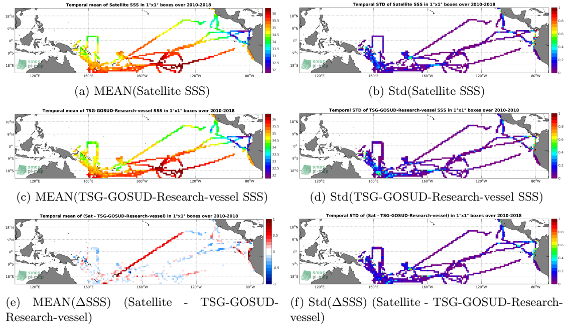
Figure 6: Temporal mean (left) and Std (right) of SSS from CCI L4 Merged-OI v1.8 - 7-day running (ESA) (top), TSG-GOSUD-Research-vessel (middle), and of \Delta SSS (Satellite - TSG-GOSUD-Research-vessel). Only match-up pairs are used to generate these maps.
