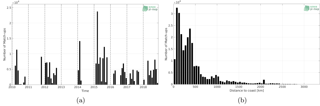
Figure 1: Number of match-ups between TSG-GOSUD-Research-vessel and CCI L4 Merged-OI v1.8 - 7-day running (ESA) SSS as a function of time (a) and as function of the distance to coast (b) over the Tropical Pacific Ocean Pi-MEP region and for the full satellite product period.
