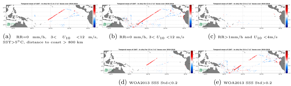
Figure 12: Temporal mean gridded over spatial boxes of size 1^\circ \times 1^\circ of \Delta SSS (CCI-L4-ESA-MERGED-OI-V1.8-7DAY-RUNNING - TSG-GOSUD-Research-vessel) for 5 different sub-datasets corresponding to: RR=0 mm/h, 3 < U_{10} < 12 m/s, SST > 5^\circ\text{C} , distance to coast > 800 km (a), RR=0 mm/h, 3 < U_{10} < 12 m/s (b), RR > 1 mm/h and U_{10} < 4 m/s (c), WOA2013 SSS Std < 0.2 (d), WOA2013 SSS Std > 0.2 (e).
