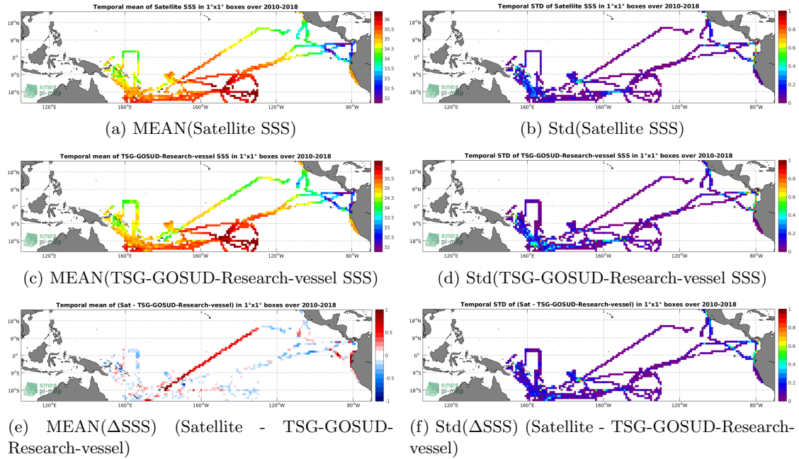
Figure 6: Temporal mean (left) and Std (right) of SSS from CCI-L4-ESA-MERGED-OI-V1.8-7DAY-RUNNING (top), TSG-GOSUD-Research-vessel (middle), and of \Delta SSS (Satellite - TSG-GOSUD-Research-vessel). Only match-up pairs are used to generate these maps.
