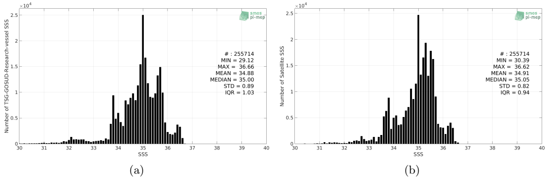
Figure 2: Histograms of SSS from TSG-GOSUD-Research-vessel (a) and CCI-L4-ESA-MERGED-OI-V1.8-7DAY-RUNNING (b) considering all match-up pairs per bins of 0.1 over the Tropical Pacific Ocean Pi-MEP region and for the full satellite product period.
