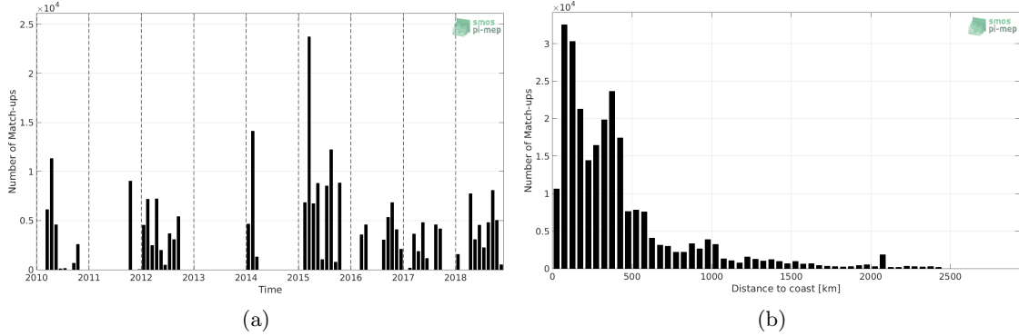
Figure 1: Number of match-ups between TSG-GOSUD-Research-vessel and CCI-L4-ESA-MERGED-OI-V1.8-7DAY-RUNNING SSS as a function of time (a) and as function of the distance to coast (b) over the Tropical Pacific Ocean Pi-MEP region and for the full satellite product period.
