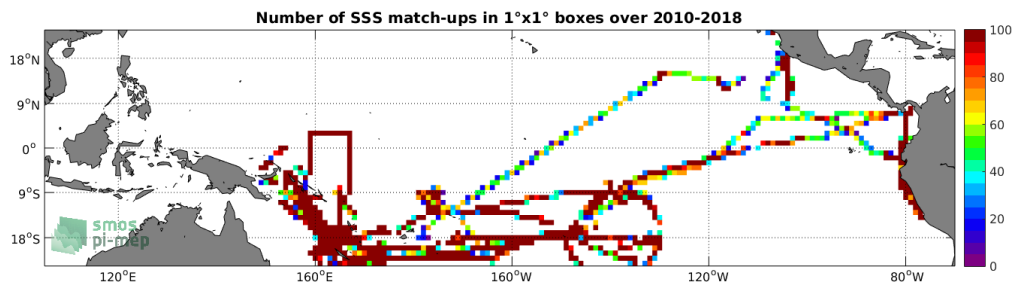
Figure 4: Number of SSS match-ups between TSG-GOSUD-Research-vessel SSS and the CCI-L4-ESA-MERGED-OI-V1.8-7DAY-RUNNING SSS product for the Tropical Pacific Ocean Pi-MEP region over 1^\circ \times 1^\circ boxes and for the full satellite product period.
