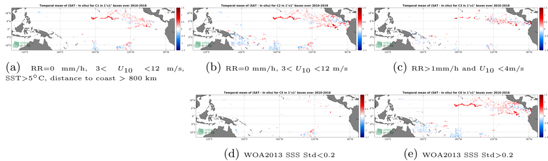
Figure 11: Temporal mean gridded over spatial boxes of size 1^\circ \times 1^\circ of \Delta SSS (CCI L4 Merged-OI v1.8 - 7-day running (ESA) - Surface drifters) for 5 different subdatasets corresponding to:RR=0 mm/h, 3 < U_{10} < 12 m/s, SST > 5^\circ C , distance to coast > 800 km (a), RR=0 mm/h, 3 < U_{10} < 12 m/s (b), RR >1 mm/h and U_{10} < 4 m/s (c), WOA2013 SSS Std <0.2 (d), WOA2013 SSS Std >0.2 (e).
