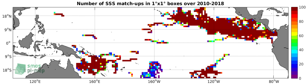
Figure 3: Number of SSS match-ups between Surface drifters SSS and the CCI L4 Merged-OI v1.8 - 7-day running (ESA) SSS product for the Tropical Pacific Ocean Pi-MEP region over 1^\circ \times 1^\circ boxes and for the full satellite product period.
