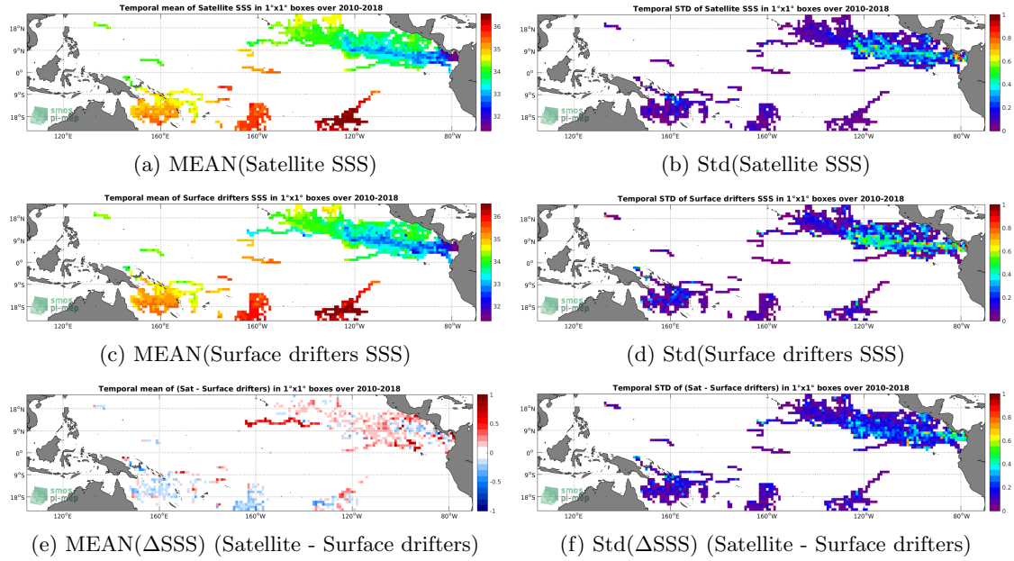
Figure 5: Temporal mean (left) and Std (right) of SSS from CCI L4 Merged-OI v1.8 - 7-day running (ESA) (top), Surface drifters (middle), and of \Delta SSS (Satellite - Surface drifters). Only match-up pairs are used to generate these maps.
