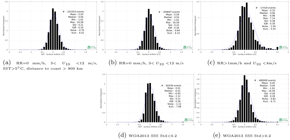
Figure 12: Normalized histogram of \Delta SSS (CCI L4 Merged-OI v1.8 - 7-day running (ESA) - Surface drifters) for 5 different subdatasets corresponding to: RR=0 mm/h, 3 < U_{10} < 12 m/s, SST>5°C, distance to coast > 800 km (a), RR=0 mm/h, 3 < U_{10} < 12 m/s (b), RR>1mm/h and U_{10} < 4 m/s (c), WOA2013 SSS Std<0.2 (d), WOA2013 SSS Std>0.2 (e).
