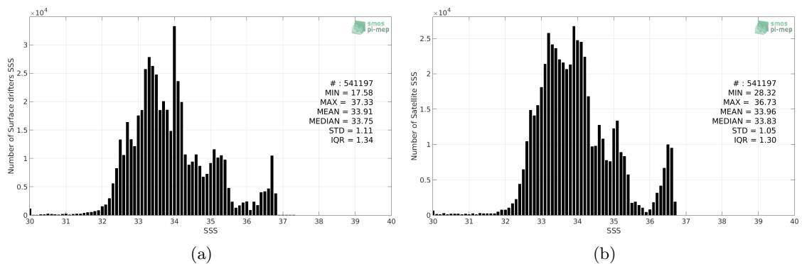
Figure 2: Histograms of SSS from Surface drifters (a) and CCI L4 Merged-OI v1.8 - 7-day running (ESA) (b) considering all match-up pairs per bins of 0.1 over the Tropical Pacific Ocean Pi-MEP region and for the full satellite product period.
