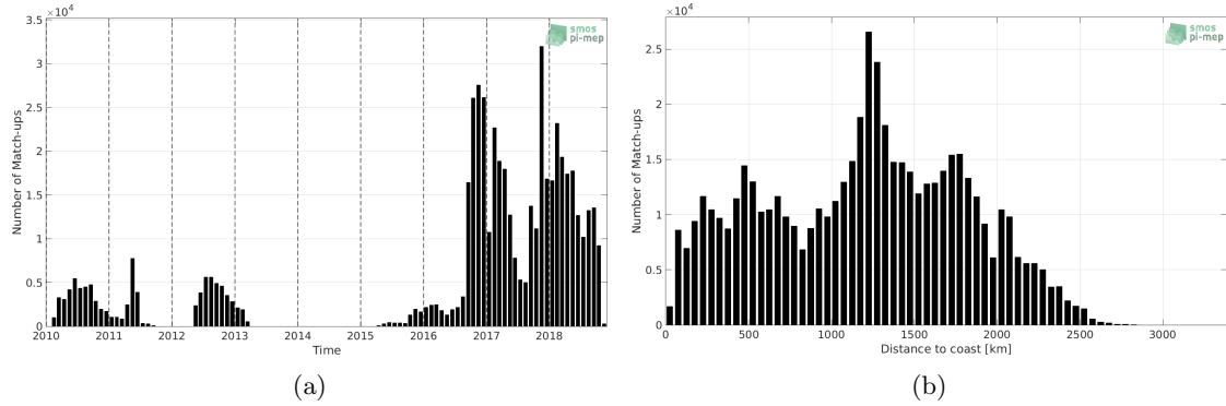
Figure 1: Number of match-ups between Surface drifters and CCI L4 Merged-OI v1.8 - 7-day running (ESA) SSS as a function of time (a) and as function of the distance to coast (b) over the Tropical Pacific Ocean Pi-MEP region and for the full satellite product period.
