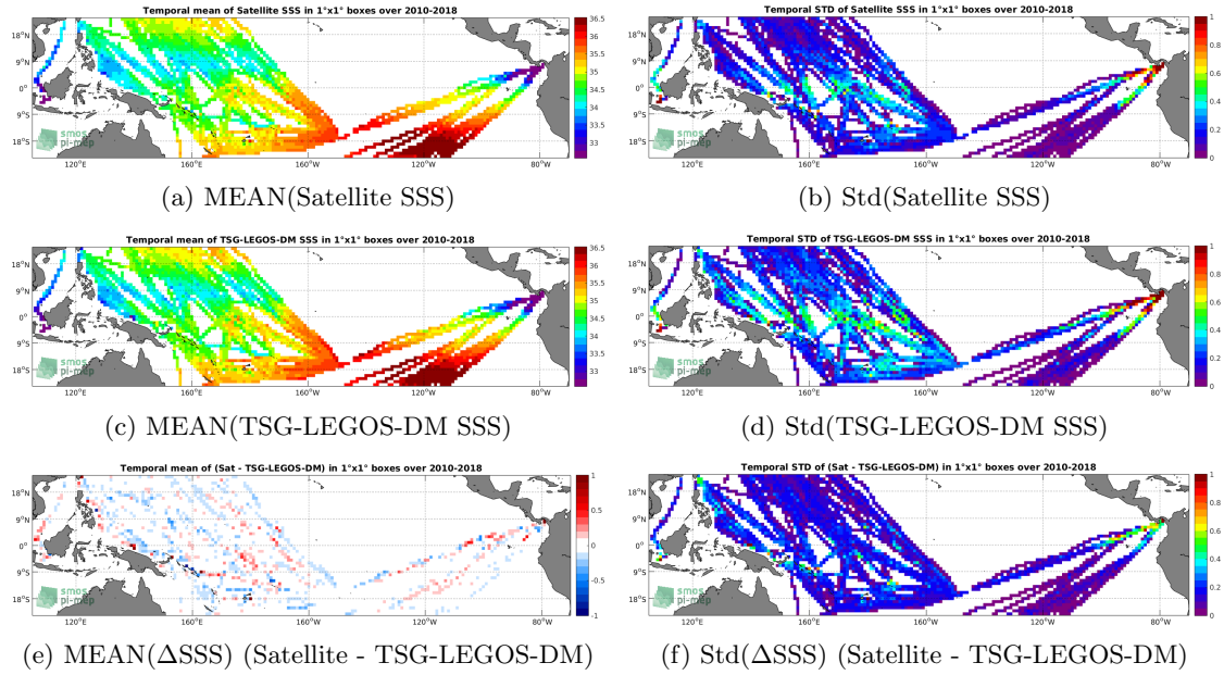
Figure 6: Temporal mean (left) and Std (right) of SSS from CCI L4 Merged-OI v1.8 - 30-day running (ESA) (top), TSG-LEGOS-DM (middle), and of \Delta SSS (Satellite - TSG-LEGOS-DM). Only match-up pairs are used to generate these maps.
