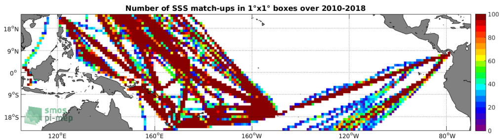
Figure 4: Number of SSS match-ups between TSG-LEGOS-DM SSS and the CCI L4 Merged-OI v1.8 - 30-day running (ESA) SSS product for the Tropical Pacific Ocean Pi-MEP region over 1°x1° boxes and for the full satellite product period.
