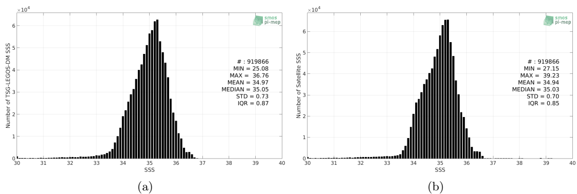
Figure 2: Histograms of SSS from TSG-LEGOS-DM (a) and CCI L4 Merged-OI v1.8 - 30-day running (ESA) (b) considering all match-up pairs per bins of 0.1 over the Tropical Pacific Ocean Pi-MEP region and for the full satellite product period.
