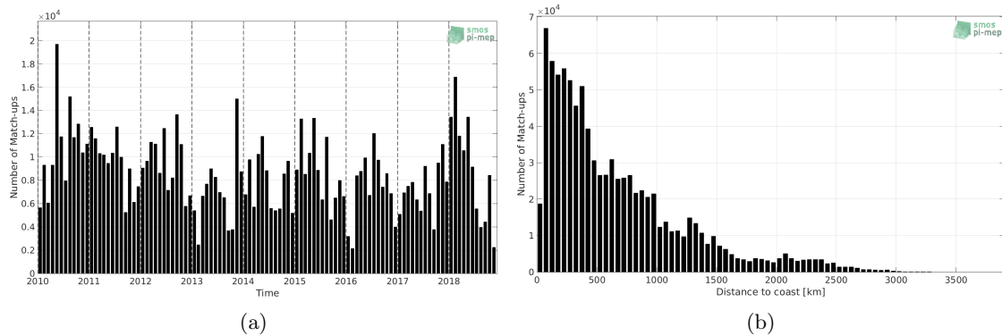
Figure 1: Number of match-ups between TSG-LEGOS-DM and CCI L4 Merged-OI v1.8 - 30-day running (ESA) SSS as a function of time (a) and as function of the distance to coast (b) over the Tropical Pacific Ocean Pi-MEP region and for the full satellite product period.
