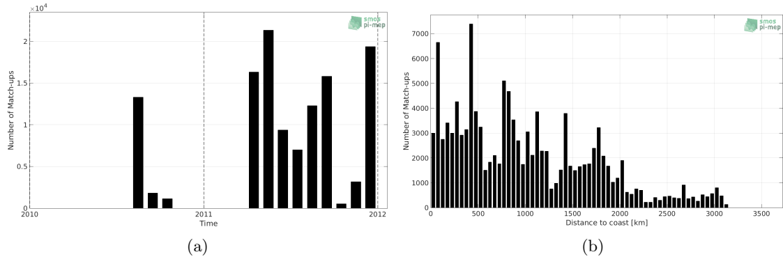
Figure 1: Number of match-ups between TSG-GOSUD-Sailing-ship and CCI-L4-ESA-MERGED-OI-V1.8-30DAY-RUNNING SSS as a function of time (a) and as function of the distance to coast (b) over the Tropical Pacific Ocean Pi-MEP region and for the full satellite product period.
