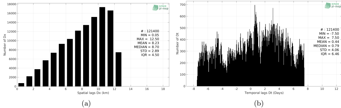
Figure 5: Histograms of the spatial (a) and temporal (b) lags between the time of the TSG-GOSUD-Sailing-ship measurements and the date of the corresponding CCI-L4-ESA-MERGED-OI-V1.8-30DAY-RUNNING SSS product.
