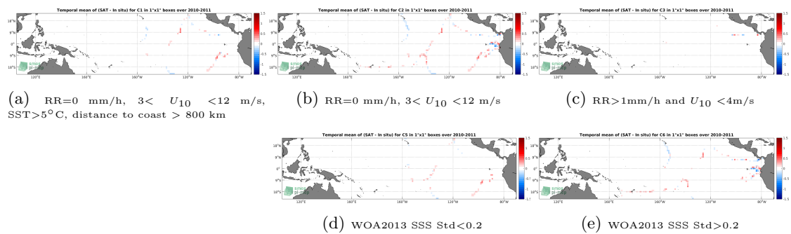
Figure 12: Temporal mean gridded over spatial boxes of size 1^\circ \times 1^\circ of \Delta SSS (CCI-L4-ESAMERGED-OI-V1.8-30DAY-RUNNING - TSG-GOSUD-Sailing-ship) for 5 different subdatasets corresponding to:RR=0 mm/h, 3 < U_{10} < 12 m/s, SST >5^\circ C, distance to coast > 800 km (a), RR=0 mm/h, 3 < U_{10} < 12 m/s (b), RR >1 mm/h and U_{10} < 4 m/s (c), WOA2013 SSS Std <0.2 (d), WOA2013 SSS Std >0.2 (e).
