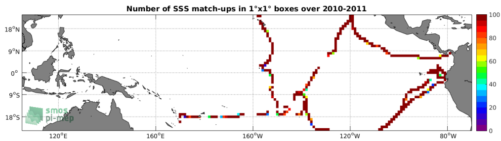
Figure 4: Number of SSS match-ups between TSG-GOSUD-Sailing-ship SSS and the CCI-L4-ESA-MERGED-OI-V1.8-30DAY-RUNNING SSS product for the Tropical Pacific Ocean Pi-MEP region over 1^\circ \times 1^\circ boxes and for the full satellite product period.
