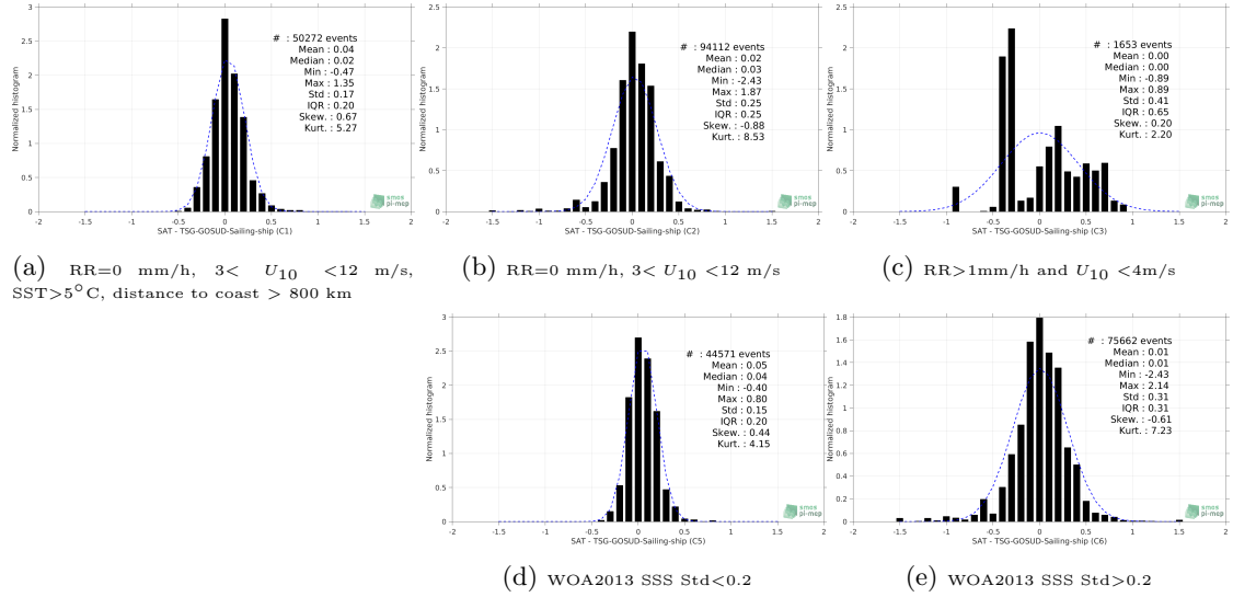
Figure 13: Normalized histogram of \Delta SSS (CCI-L4-ESA-MERGED-OI-V1.8-30DAY-RUNNING - TSG-GOSUD-Sailing-ship) for 5 different subdatasets corresponding to: RR=0 mm/h, 3 < U_{10} < 12 m/s, SST > 5°C, distance to coast > 800 km (a), RR=0 mm/h, 3 < U_{10} < 12 m/s (b), RR > 1mm/h and U_{10} < 4 m/s (c), WOA2013 SSS Std < 0.2 (d), WOA2013 SSS Std > 0.2 (e).
