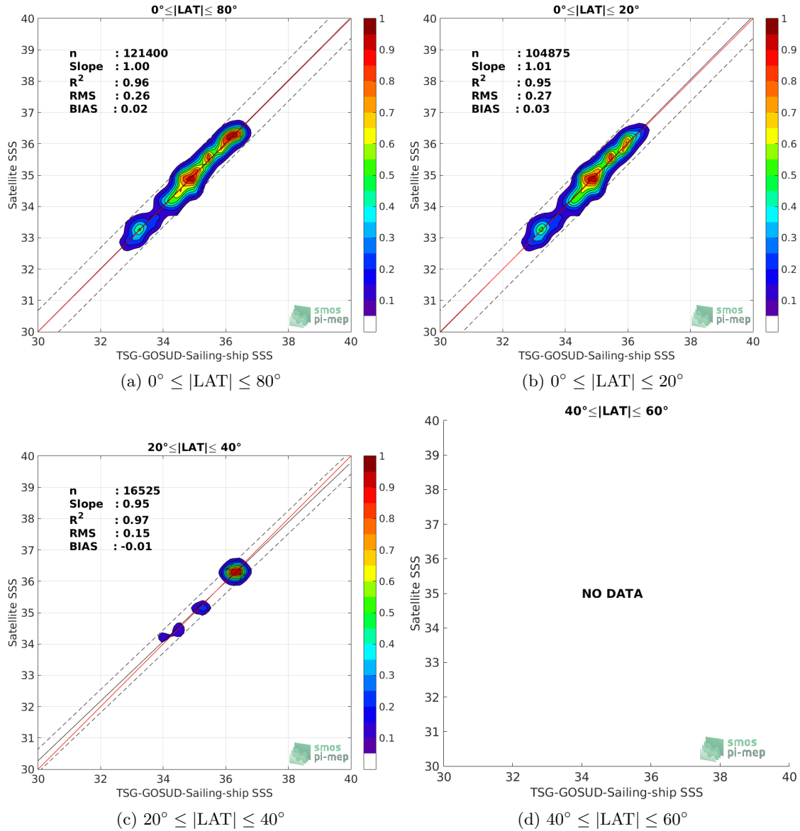
Figure 9: Contour maps of the concentration of CCI-L4-ESA-MERGED-OI-V1.8-30DAY-RUNNING SSS (y-axis) versus TSG-GOSUD-Sailing-ship SSS (x-axis) at match-up pairs for different latitude bands. For each plot, the red line shows x=y . The black thin and dashed lines indicate a linear fit through the data cloud and the \pm 95\% confidence levels, respectively. The number match-up pairs n , the slope and R^2 coefficient of the linear fit, the root mean square (RMS) and the mean bias between satellite and in situ data are indicated for each latitude band in each plots.
