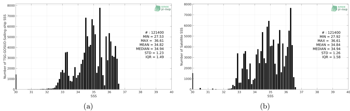
Figure 2: Histograms of SSS from TSG-GOSUD-Sailing-ship (a) and CCI-L4-ESA-MERGED-OI-V1.8-30DAY-RUNNING (b) considering all match-up pairs per bins of 0.1 over the Tropical Pacific Ocean Pi-MEP region and for the full satellite product period.
