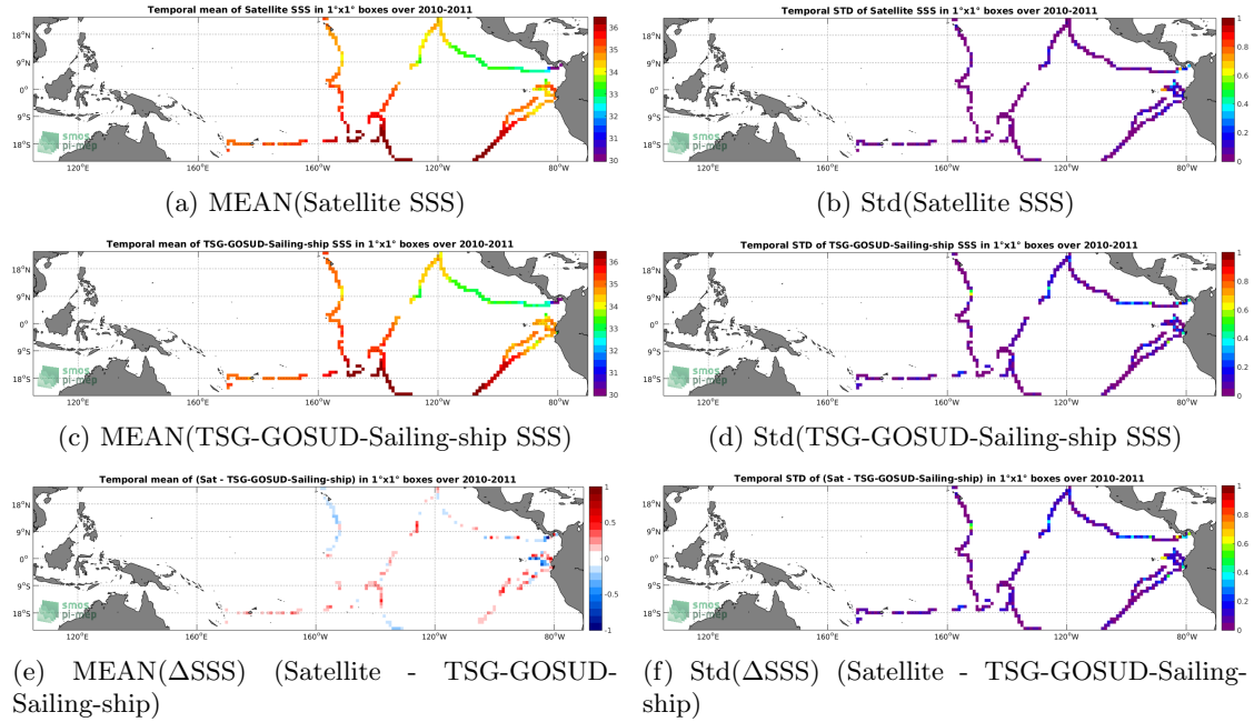
Figure 6: Temporal mean (left) and Std (right) of SSS from CCI-L4-ESA-MERGED-OI-V1.8-30DAY-RUNNING (top), TSG-GOSUD-Sailing-ship (middle), and of \Delta SSS (Satellite - TSG-GOSUD-Sailing-ship). Only match-up pairs are used to generate these maps.
