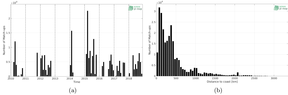
Figure 1: Number of match-ups between TSG-GOSUD-Research-vessel and CCI L4 Merged-OI v1.8 - 30-day running (ESA) SSS as a function of time (a) and as function of the distance to coast (b) over the Tropical Pacific Ocean Pi-MEP region and for the full satellite product period.
