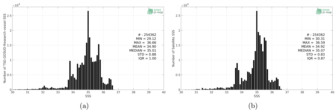
Figure 2: Histograms of SSS from TSG-GOSUD-Research-vessel (a) and CCI L4 Merged-OI v1.8 - 30-day running (ESA) (b) considering all match-up pairs per bins of 0.1 over the Tropical Pacific Ocean Pi-MEP region and for the full satellite product period.
