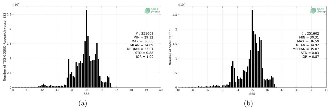
Figure 2: Histograms of SSS from TSG-GOSUD-Research-vessel (a) and CCI-L4-ESA-MERGED-OI-V1.8-30DAY-RUNNING (b) considering all match-up pairs per bins of 0.1 over the Tropical Pacific Ocean Pi-MEP region and for the full satellite product period.
