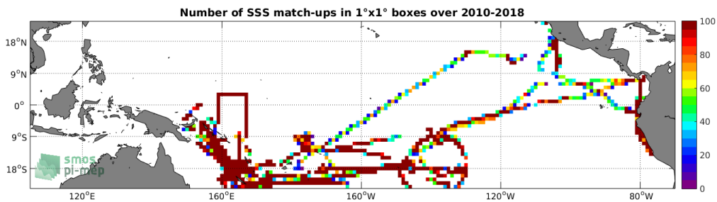
Figure 4: Number of SSS match-ups between TSG-GOSUD-Research-vessel SSS and the CCI-L4-ESA-MERGED-OI-V1.8-30DAY-RUNNING SSS product for the Tropical Pacific Ocean Pi-MEP region over 1^\circ \times 1^\circ boxes and for the full satellite product period.
