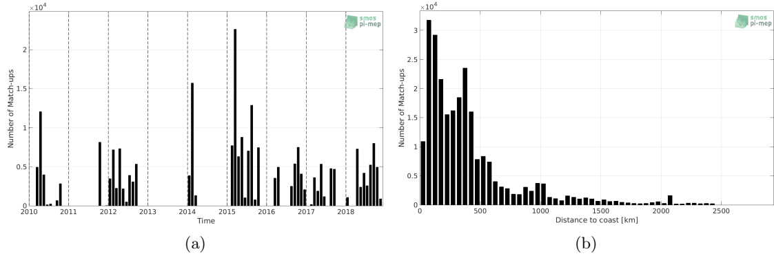
Figure 1: Number of match-ups between TSG-GOSUD-Research-vessel and CCI-L4-ESA-MERGED-OI-V1.8-30DAY-RUNNING SSS as a function of time (a) and as function of the distance to coast (b) over the Tropical Pacific Ocean Pi-MEP region and for the full satellite product period.
