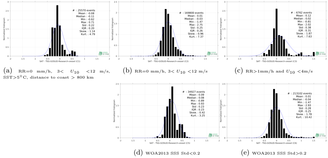
Figure 13: Normalized histogram of \Delta SSS (CCI-L4-ESA-MERGED-OI-V1.8-30DAY-RUNNING - TSG-GOSUD-Research-vessel) for 5 different subdatasets corresponding to: RR=0 mm/h, 3 < U_{10} < 12 m/s, SST>5°C, distance to coast > 800 km (a), RR=0 mm/h, 3 < U_{10} < 12 m/s (b), RR>1mm/h and U_{10} < 4 m/s (c), WOA2013 SSS Std<0.2 (d), WOA2013 SSS Std>0.2 (e).
