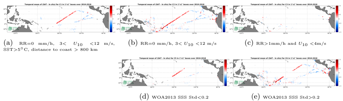
Figure 12: Temporal mean gridded over spatial boxes of size 1^\circ \times 1^\circ of \Delta SSS (CCI-L4-ESA-MERGED-OI-V1.8-30DAY-RUNNING - TSG-GOSUD-Research-vessel) for 5 different sub-datasets corresponding to: RR=0 mm/h, 3 < U_{10} < 12 m/s, SST > 5°C, distance to coast > 800 km (a), RR=0 mm/h, 3 < U_{10} < 12 m/s (b), RR > 1mm/h and U_{10} < 4 m/s (c), WOA2013 SSS Std < 0.2 (d), WOA2013 SSS Std > 0.2 (e).
