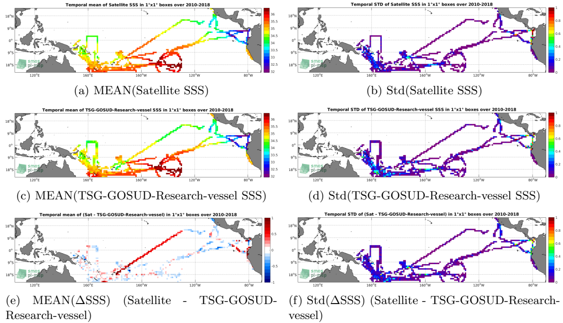
Figure 6: Temporal mean (left) and Std (right) of SSS from CCI-L4-ESA-MERGED-OI-V1.8-30DAY-RUNNING (top), TSG-GOSUD-Research-vessel (middle), and of \Delta SSS (Satellite - TSG-GOSUD-Research-vessel). Only match-up pairs are used to generate these maps.
