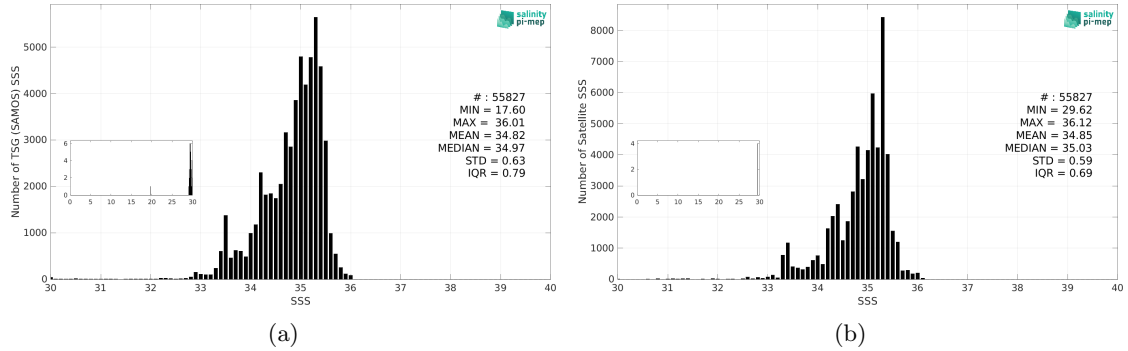
Figure 3: Histograms of SSS from TSG (SAMOS) (a) and Aquarius SSS L4 OI v5 - Weekly (IPRC) (b) considering all match-up pairs per bins of 0.1 over the Tropical Pacific Ocean Pi-MEP region and for the full satellite product period.
