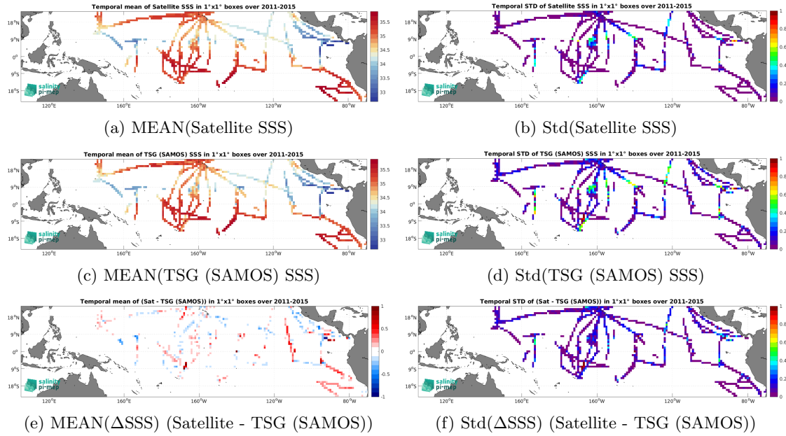
Figure 7: Temporal mean (left) and Std (right) of SSS from Aquarius SSS L4 OI v5 - Weekly (IPRC) (top), TSG (SAMOS) (middle), and of \Delta SSS (Satellite - TSG (SAMOS)). Only match-up pairs are used to generate these maps.
