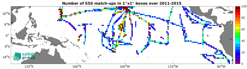
Figure 5: Number of SSS match-ups between TSG (SAMOS) SSS and the Aquarius SSS L4 OI v5 - Weekly (IPRC) SSS product for the Tropical Pacific Ocean Pi-MEP region over 1^\circ \times 1^\circ boxes and for the full satellite product period.
