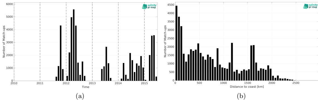
Figure 2: Number of match-ups between TSG (SAMOS) and Aquarius SSS L4 OI v5 - Weekly (IPRC) SSS as a function of time (a) and as function of the distance to coast (b) over the Tropical Pacific Ocean Pi-MEP region and for the full satellite product period.
