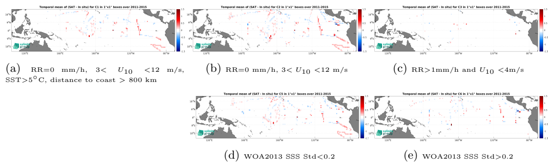
Figure 14: Temporal mean gridded over spatial boxes of size 1^\circ \times 1^\circ of \Delta SSS (Aquarius SSS L4 OI v5 - Weekly (IPRC) - TSG (SAMOS)) for 5 different subdatasets corresponding to: RR=0 mm/h, 3 < U_{10} < 12 m/s, SST > 5°C, distance to coast > 800 km (a), RR=0 mm/h, 3 < U_{10} < 12 m/s (b), RR > 1mm/h and U_{10} < 4 m/s (c), WOA2013 SSS Std < 0.2 (d), WOA2013 SSS Std > 0.2 (e).
