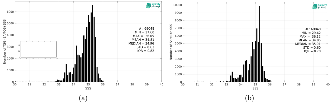
Figure 2: Histograms of SSS from TSG (SAMOS) (a) and Aquarius SSS L4 OI v5 - Weekly (IPRC) (b) considering all match-up pairs per bins of 0.1 over the Tropical Pacific Ocean Pi-MEP region and for the full satellite product period.
