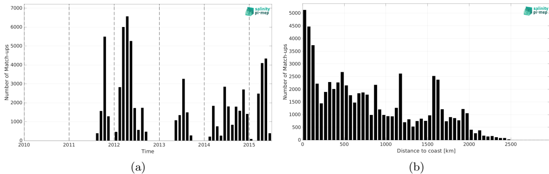
Figure 1: Number of match-ups between TSG (SAMOS) and Aquarius SSS L4 OI v5 - Weekly (IPRC) SSS as a function of time (a) and as function of the distance to coast (b) over the Tropical Pacific Ocean Pi-MEP region and for the full satellite product period.
