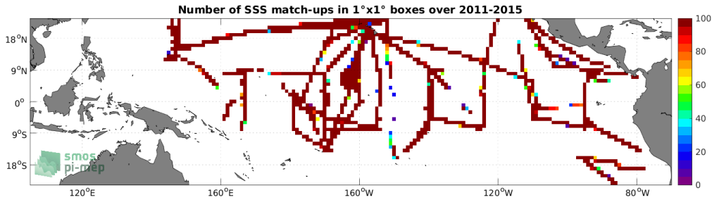
Figure 4: Number of SSS match-ups between TSG (SAMOS) SSS and the Aquarius SSS L4 OI v5 - Weekly (IPRC) SSS product for the Tropical Pacific Ocean Pi-MEP region over 1^\circ \times 1^\circ boxes and for the full satellite product period.
