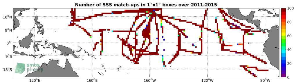
Figure 4: Number of SSS match-ups between TSG (SAMOS) SSS and the Aquarius SSS L4 OI v5 - Weekly (IPRC) SSS product for the Tropical Pacific Ocean Pi-MEP region over 1^\circ \times 1^\circ boxes and for the full satellite product period.
