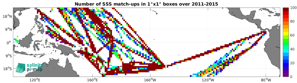
Figure 4: Number of SSS match-ups between TSG (LEGOS-DM) SSS and the Aquarius SSS L4 OI v5 - Weekly (IPRC) SSS product for the Tropical Pacific Ocean Pi-MEP region over 1^\circ \times 1^\circ boxes and for the full satellite product period.
