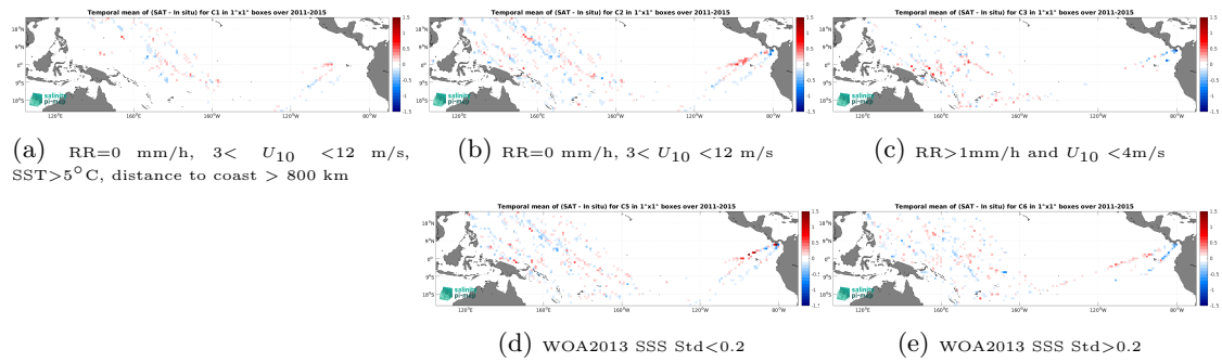
Figure 12: Temporal mean gridded over spatial boxes of size 1^\circ \times 1^\circ of \Delta\text{SSS} (Aquarius SSS L4 OI v5 - Weekly (IPRC) - TSG (LEGOS-DM)) for 5 different subdatasets corresponding to: RR=0 mm/h, 3 < U_{10} < 12 m/s, SST > 5^\circ\text{C} , distance to coast > 800 km (a), RR=0 mm/h, 3 < U_{10} < 12 m/s (b), RR > 1\text{mm/h} and U_{10} < 4\text{m/s} (c), WOA2013 SSS Std < 0.2 (d), WOA2013 SSS Std > 0.2 (e).
