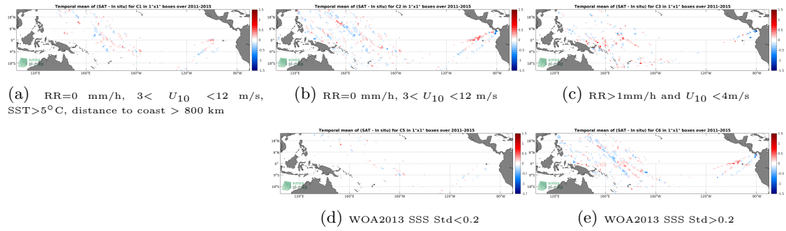
Figure 12: Temporal mean gridded over spatial boxes of size 1^\circ \times 1^\circ of \Delta SSS (Aquarius SSS L4 OI v5 - Weekly (IPRC) - TSG (LEGOS-DM)) for 5 different subdatasets corresponding to: RR=0 mm/h, 3 < U_{10} < 12 m/s, SST > 5^\circ\text{C} , distance to coast > 800 km (a), RR=0 mm/h, 3 < U_{10} < 12 m/s (b), RR > 1 mm/h and U_{10} < 4 m/s (c), WOA2013 SSS Std < 0.2 (d), WOA2013 SSS Std > 0.2 (e).
