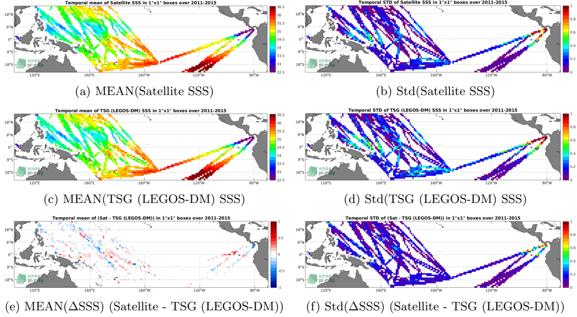
Figure 6: Temporal mean (left) and Std (right) of SSS from Aquarius SSS L4 OI v5 - Weekly (IPRC) (top), TSG (LEGOS-DM) (middle), and of \Delta SSS (Satellite - TSG (LEGOS-DM)). Only match-up pairs are used to generate these maps.
