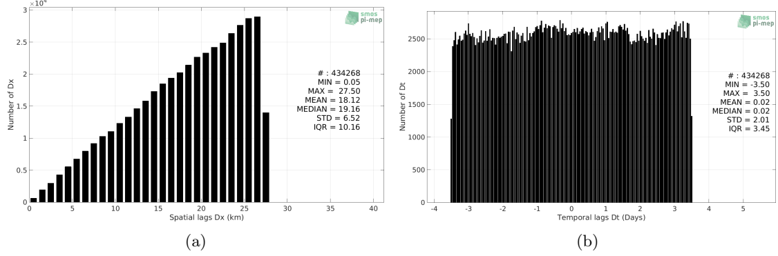
Figure 5: Histograms of the spatial (a) and temporal (b) lags between the time of the TSG (LEGOS-DM) measurements and the date of the corresponding Aquarius SSS L4 OI v5 - Weekly (IPRC) SSS product.
