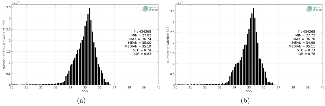
Figure 2: Histograms of SSS from TSG (LEGOS-DM) (a) and Aquarius SSS L4 OI v5 - Weekly (IPRC) (b) considering all match-up pairs per bins of 0.1 over the Tropical Pacific Ocean Pi-MEP region and for the full satellite product period.
