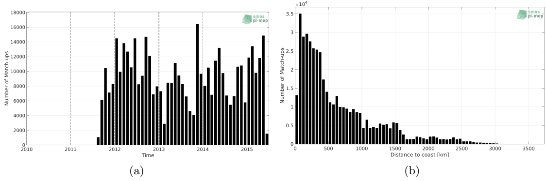
Figure 1: Number of match-ups between TSG (LEGOS-DM) and Aquarius SSS L4 OI v5 - Weekly (IPRC) SSS as a function of time (a) and as function of the distance to coast (b) over the Tropical Pacific Ocean Pi-MEP region and for the full satellite product period.
