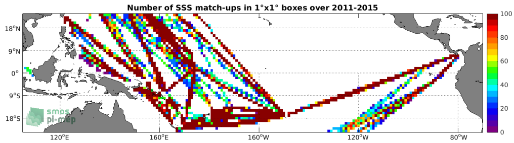
Figure 4: Number of SSS match-ups between TSG (LEGOS-DM) SSS and the Aquarius SSS L4 OI v5 - Weekly (IPRC) SSS product for the Tropical Pacific Ocean Pi-MEP region over 1°x1° boxes and for the full satellite product period.
