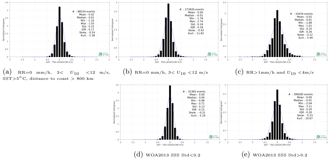
Figure 13: Normalized histogram of \Delta SSS (Aquarius-L4-IPRC-V5-WEEKLY - TSG-LEGOS-DM) for 5 different subdatasets corresponding to: RR=0 mm/h, 3 < U_{10} < 12 m/s, SST > 5^\circ C , distance to coast > 800 km (a), RR=0 mm/h, 3 < U_{10} < 12 m/s (b), RR > 1 mm/h and U_{10} < 4 m/s (c), WOA2013 SSS Std <0.2 (d), WOA2013 SSS Std >0.2 (e).
