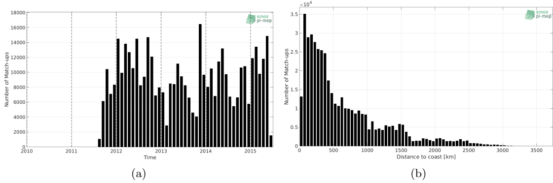
Figure 1: Number of match-ups between TSG-LEGOS-DM and Aquarius-L4-IPRC-V5-WEEKLY SSS as a function of time (a) and as function of the distance to coast (b) over the Tropical Pacific Ocean Pi-MEP region and for the full satellite product period.
