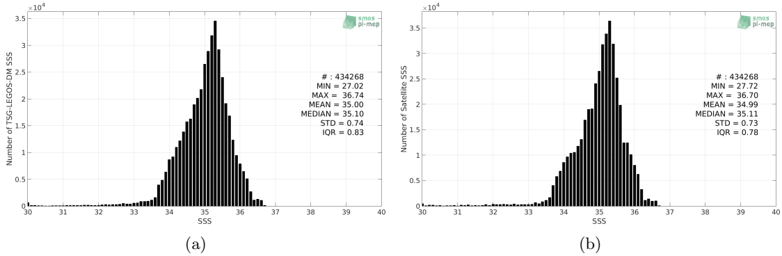
Figure 2: Histograms of SSS from TSG-LEGOS-DM (a) and Aquarius-L4-IPRC-V5-WEEKLY (b) considering all match-up pairs per bins of 0.1 over the Tropical Pacific Ocean Pi-MEP region and for the full satellite product period.
