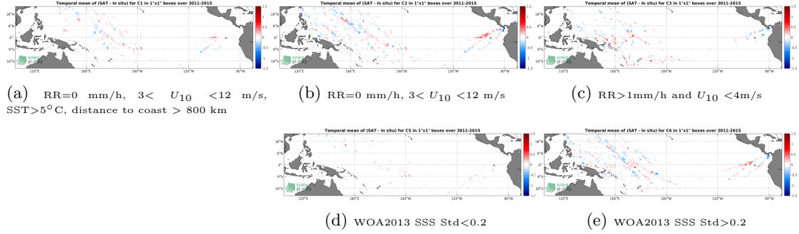
Figure 12: Temporal mean gridded over spatial boxes of size 1^\circ \times 1^\circ of \Delta SSS (Aquarius-L4-IPRC-V5-WEEKLY - TSG-LEGOS-DM) for 5 different subdatasets corresponding to: RR=0 mm/h, 3 < U_{10} < 12 m/s, SST > 5^\circ C , distance to coast > 800 km (a), RR=0 mm/h, 3 < U_{10} < 12 m/s (b), RR > 1 mm/h and U_{10} < 4 m/s (c), WOA2013 SSS Std <0.2 (d), WOA2013 SSS Std >0.2 (e).
