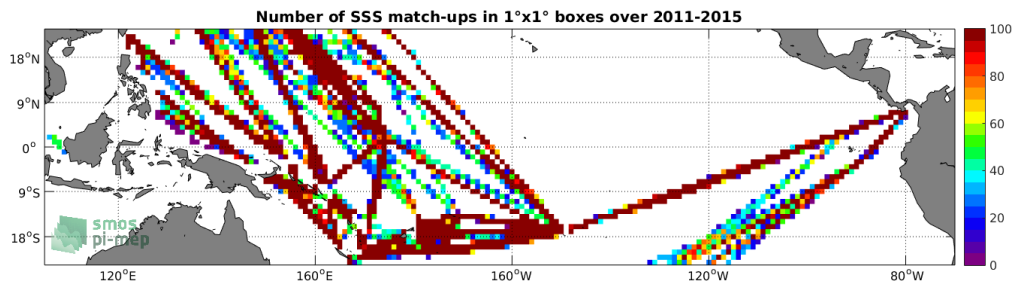
Figure 4: Number of SSS match-ups between TSG-LEGOS-DM SSS and the Aquarius-L4-IPRC-V5-WEEKLY SSS product for the Tropical Pacific Ocean Pi-MEP region over 1°x1° boxes and for the full satellite product period.
