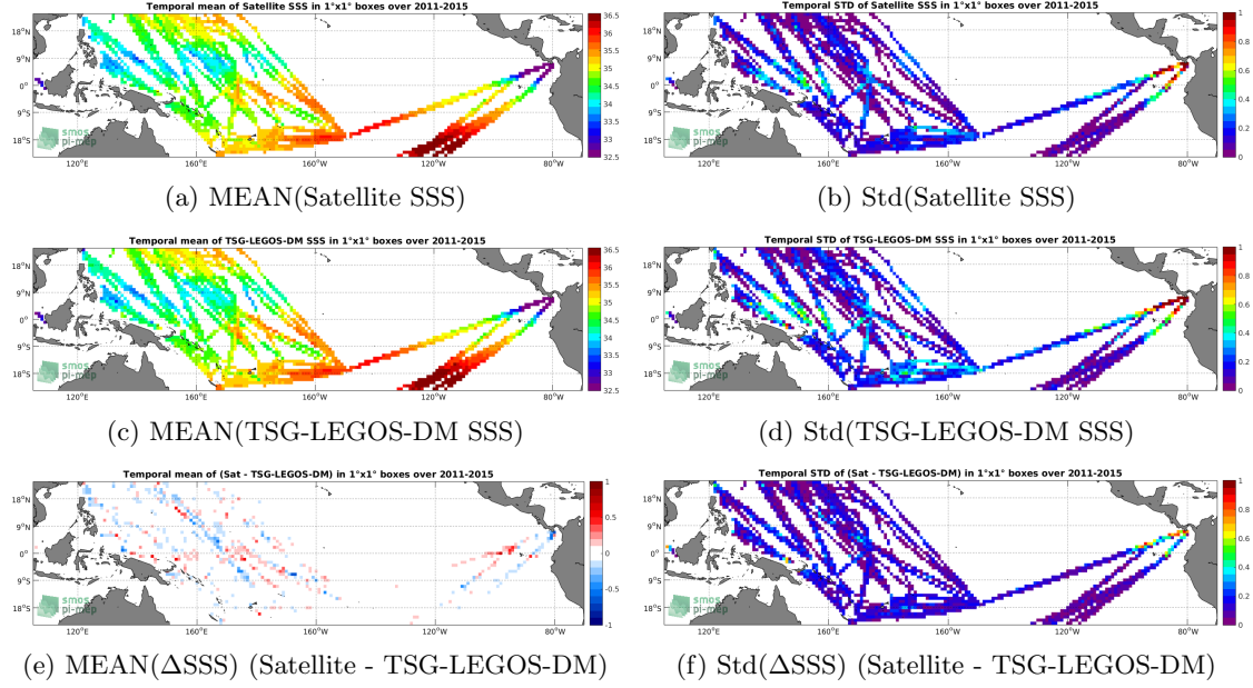
Figure 6: Temporal mean (left) and Std (right) of SSS from Aquarius-L4-IPRC-V5-WEEKLY (top), TSG-LEGOS-DM (middle), and of \Delta SSS (Satellite - TSG-LEGOS-DM). Only match-up pairs are used to generate these maps.
