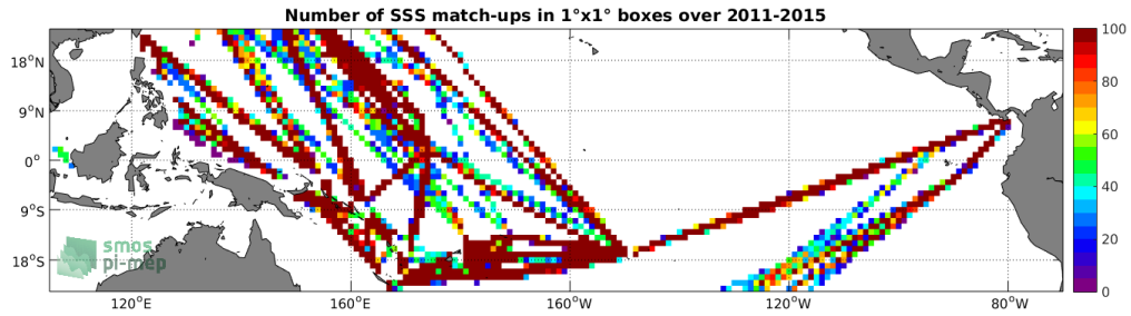
Figure 4: Number of SSS match-ups between TSG-LEGOS-DM SSS and the Aquarius-L4-IPRC-V5-WEEKLY SSS product for the Tropical Pacific Ocean Pi-MEP region over 1^\circ \times 1^\circ boxes and for the full satellite product period.
