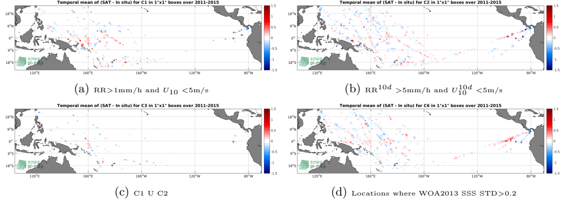
Figure 12: Temporal mean gridded over spatial boxes of size 1^\circ \times 1^\circ of \Delta SSS (Aquarius-L4-IPRC-V5-WEEKLY - TSG-LEGOS-DM) for 4 different subdatasets corresponding to: RR > 1mm/h and U_{10} < 5\text{m/s} (a), RR^{10d} > 5\text{mm/h} and U_{10}^{10d} < 5\text{m/s} (b), C1 U C2 (c), Locations where WOA2013 SSS STD > 0.2 (d).
