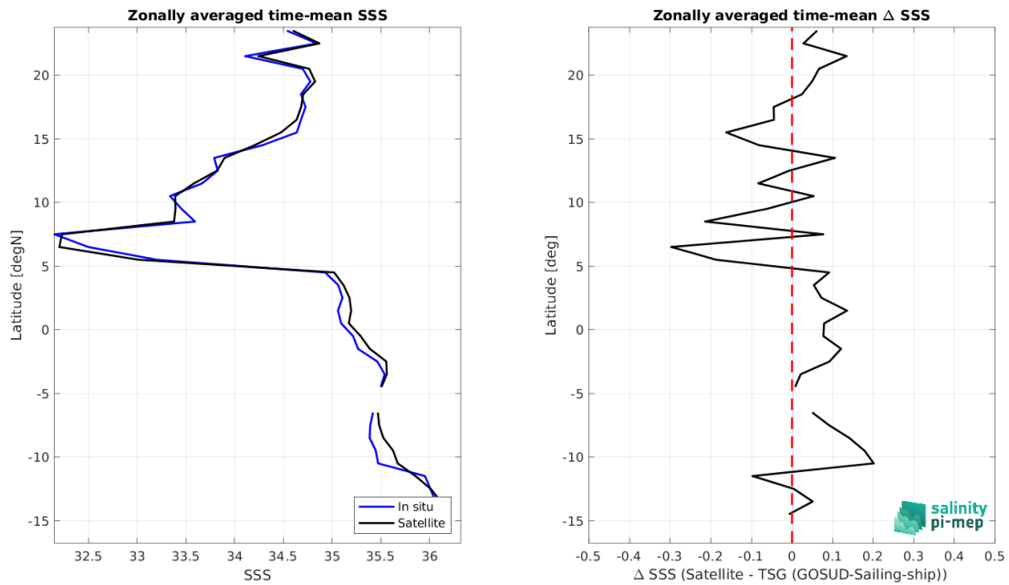
Figure 9: Left panel: Zonal mean SSS from Aquarius SSS L4 OI v5 - Weekly (IPRC) satellite product (black) and from TSG (GOSUD-Sailing-ship) (blue). Right panel: Zonal mean of \Delta SSS (Satellite - TSG (GOSUD-Sailing-ship)) for all the collected Pi-MEP match-up pairs estimated over the full satellite product period.
