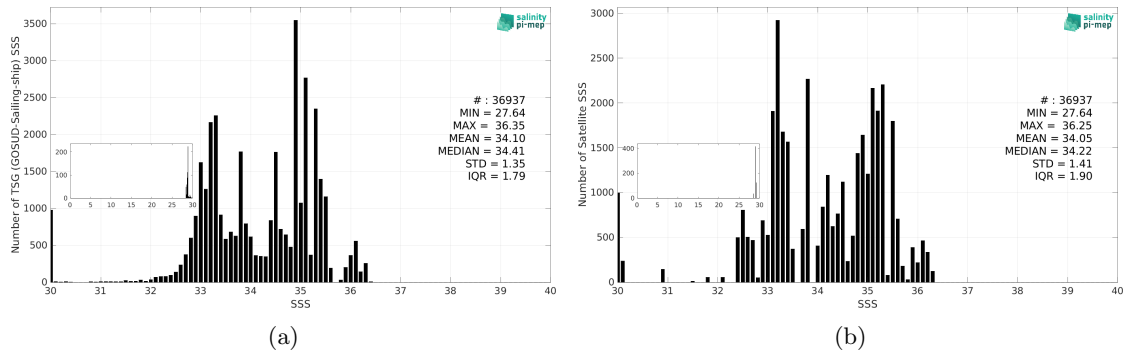
Figure 3: Histograms of SSS from TSG (GOSUD-Sailing-ship) (a) and Aquarius SSS L4 OI v5 - Weekly (IPRC) (b) considering all match-up pairs per bins of 0.1 over the Tropical Pacific Ocean Pi-MEP region and for the full satellite product period.
