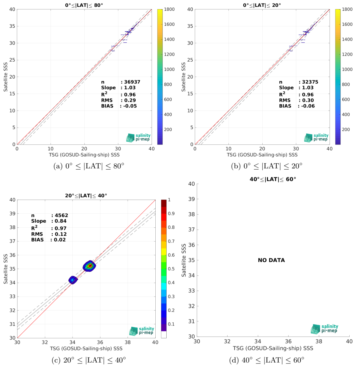
Figure 10: Contour maps of the concentration of Aquarius SSS L4 OI v5 - Weekly (IPRC) SSS (y-axis) versus TSG (GOSUD-Sailing-ship) SSS (x-axis) at match-up pairs for different latitude bands. For each plot, the red line shows x=y . The black thin and dashed lines indicate a linear fit through the data cloud and the \pm 95\% confidence levels, respectively. The number match-up pairs n , the slope and R^2 coefficient of the linear fit, the root mean square (RMS) and the mean bias between satellite and in situ data are indicated for each latitude band in each plots.
