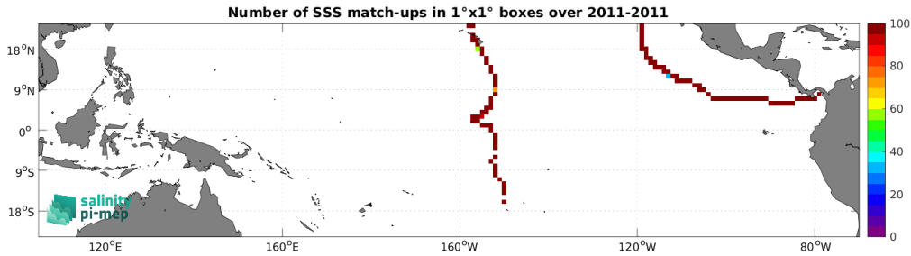
Figure 5: Number of SSS match-ups between TSG (GOSUD-Sailing-ship) SSS and the Aquarius SSS L4 OI v5 - Weekly (IPRC) SSS product for the Tropical Pacific Ocean Pi-MEP region over 1^\circ \times 1^\circ boxes and for the full satellite product period.
