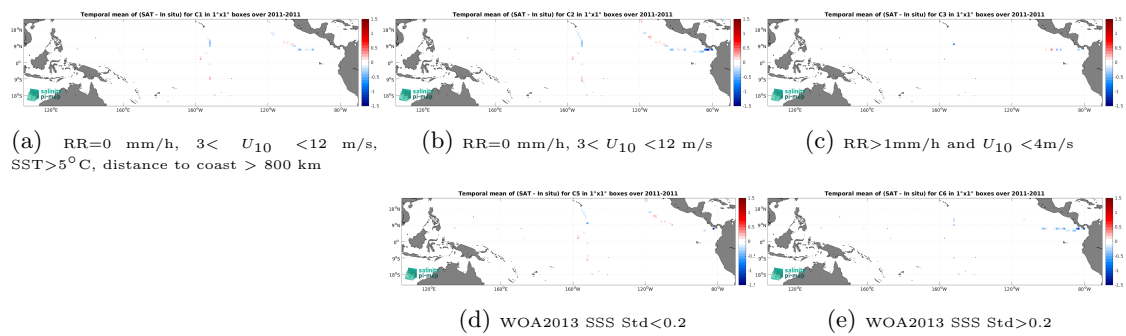
Figure 14: Temporal mean gridded over spatial boxes of size 1^\circ \times 1^\circ of \Delta SSS (Aquarius SSS L4 OI v5 - Weekly (IPRC) - TSG (GOSUD-Sailing-ship)) for 5 different subdatasets corresponding to: RR=0 mm/h, 3 < U_{10} < 12 m/s, SST > 5°C, distance to coast > 800 km (a), RR=0 mm/h, 3 < U_{10} < 12 m/s (b), RR > 1mm/h and U_{10} < 4 m/s (c), WOA2013 SSS Std < 0.2 (d), WOA2013 SSS Std > 0.2 (e).
