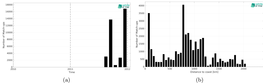
Figure 2: Number of match-ups between TSG (GOSUD-Sailing-ship) and Aquarius SSS L4 OI v5 - Weekly (IPRC) SSS as a function of time (a) and as function of the distance to coast (b) over the Tropical Pacific Ocean Pi-MEP region and for the full satellite product period.
