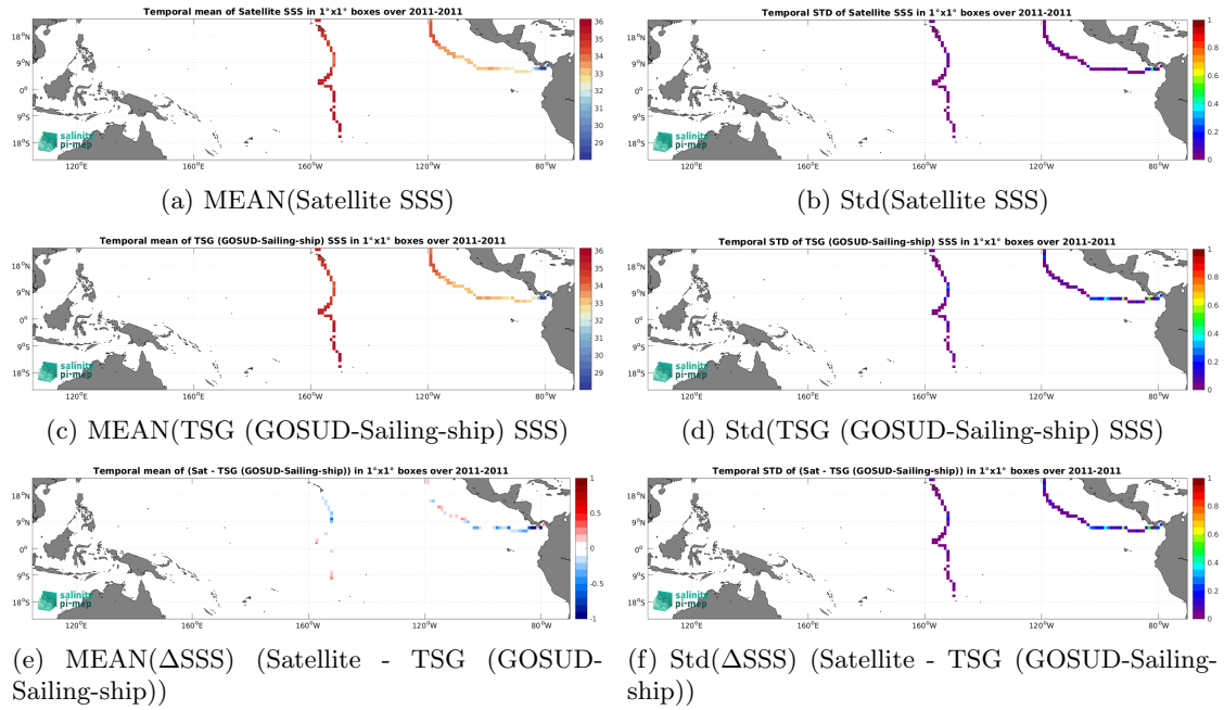
Figure 7: Temporal mean (left) and Std (right) of SSS from Aquarius SSS L4 OI v5 - Weekly (IPRC) (top), TSG (GOSUD-Sailing-ship) (middle), and of \Delta SSS (Satellite - TSG (GOSUD-Sailing-ship)). Only match-up pairs are used to generate these maps.
