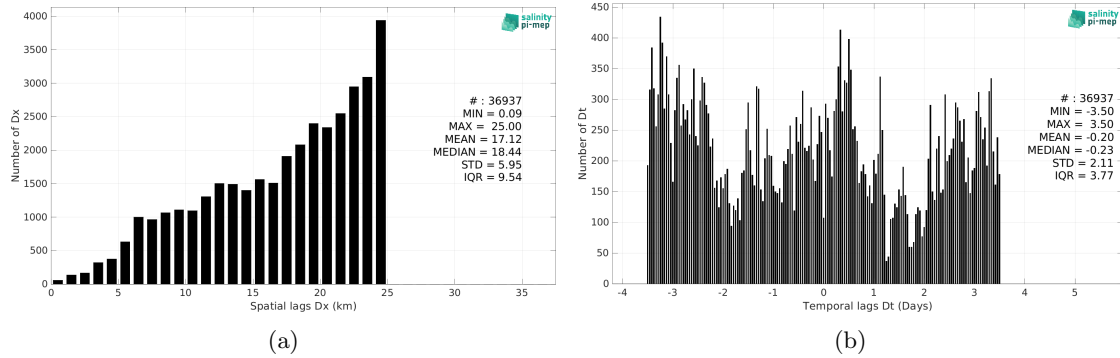
Figure 6: Histograms of the spatial (a) and temporal (b) lags between the location/time of the TSG (GOSUD-Sailing-ship) measurement and the date of the corresponding Aquarius SSS L4 OI v5 - Weekly (IPRC) SSS pixel.
