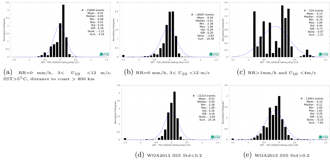
Figure 15: Normalized histogram of \Delta\text{SSS} (Aquarius SSS L4 OI v5 - Weekly (IPRC) - TSG (GOSUD-Sailing-ship)) for 5 different subdatasets corresponding to: RR=0 mm/h, 3 < U_{10} < 12 m/s, SST > 5^\circ\text{C} , distance to coast > 800 km (a), RR=0 mm/h, 3 < U_{10} < 12 m/s (b), RR > 1 mm/h and U_{10} < 4 m/s (c), WOA2013 SSS Std < 0.2 (d), WOA2013 SSS Std > 0.2 (e).
