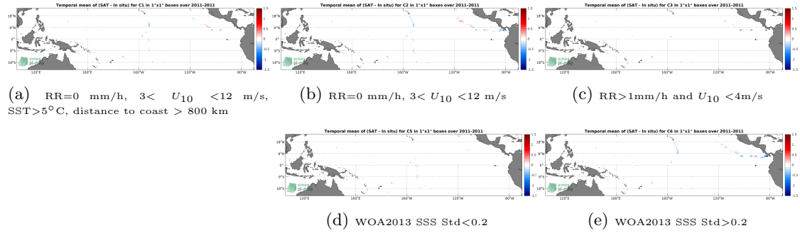
Figure 12: Temporal mean gridded over spatial boxes of size 1^\circ \times 1^\circ of \Delta SSS (Aquarius SSS L4 OI v5 - Weekly (IPRC) - TSG (GOSUD-Sailing-ship)) for 5 different subdatasets corresponding to: RR=0 mm/h, 3 < U_{10} < 12 m/s, SST > 5^\circ C , distance to coast > 800 km (a), RR=0 mm/h, 3 < U_{10} < 12 m/s (b), RR > 1 mm/h and U_{10} < 4 m/s (c), WOA2013 SSS Std < 0.2 (d), WOA2013 SSS Std > 0.2 (e).
