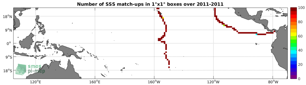
Figure 4: Number of SSS match-ups between TSG-GOSUD-Sailing-ship SSS and the Aquarius-L4-IPRC-V5-WEEKLY SSS product for the Tropical Pacific Ocean Pi-MEP region over 1°x1° boxes and for the full satellite product period.
