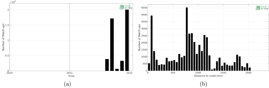
Figure 1: Number of match-ups between TSG-GOSUD-Sailing-ship and Aquarius-L4-IPRC-V5-WEEKLY SSS as a function of time (a) and as function of the distance to coast (b) over the Tropical Pacific Ocean Pi-MEP region and for the full satellite product period.
