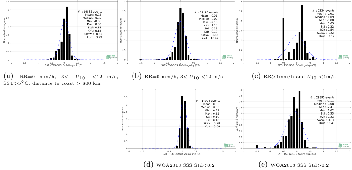
Figure 13: Normalized histogram of \Delta\text{SSS} (Aquarius-L4-IPRC-V5-WEEKLY - TSG-GOSUD-Sailing-ship) for 5 different subdatasets corresponding to: RR=0 mm/h, 3 < U_{10} < 12 m/s, SST >5^{\circ}\text{C} , distance to coast > 800 km (a), RR=0 mm/h, 3 < U_{10} < 12 m/s (b), RR>1\text{mm/h} and U_{10} < 4\text{m/s} (c), WOA2013 SSS Std <0.2 (d), WOA2013 SSS Std >0.2 (e).
