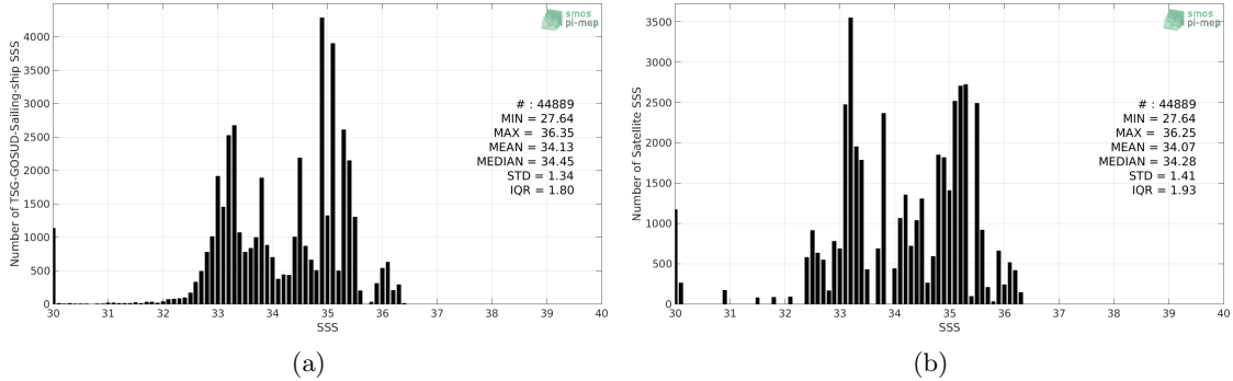
Figure 2: Histograms of SSS from TSG-GOSUD-Sailing-ship (a) and Aquarius-L4-IPRC-V5-WEEKLY (b) considering all match-up pairs per bins of 0.1 over the Tropical Pacific Ocean Pi-MEP region and for the full satellite product period.
