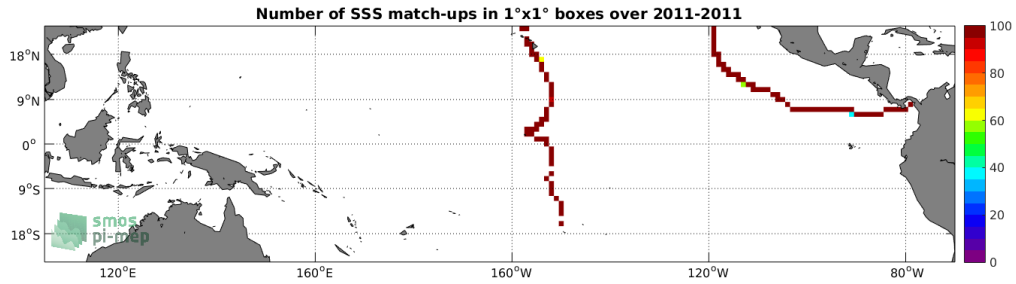
Figure 4: Number of SSS match-ups between TSG-GOSUD-Sailing-ship SSS and the Aquarius-L4-IPRC-V5-WEEKLY SSS product for the Tropical Pacific Ocean Pi-MEP region over 1^\circ \times 1^\circ boxes and for the full satellite product period.
