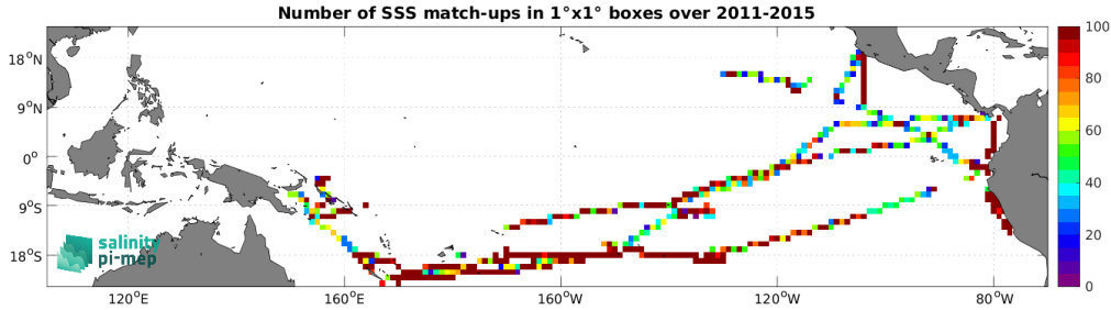
Figure 5: Number of SSS match-ups between TSG (GOSUD-Research-vessel) SSS and the Aquarius SSS L4 OI v5 - Weekly (IPRC) SSS product for the Tropical Pacific Ocean Pi-MEP region over 1^\circ \times 1^\circ boxes and for the full satellite product period.
