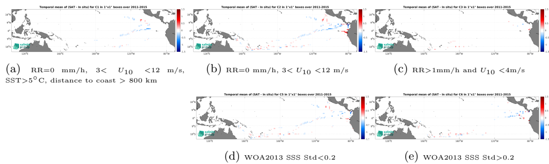
Figure 14: Temporal mean gridded over spatial boxes of size 1^\circ \times 1^\circ of \Delta SSS (Aquarius SSS L4 OI v5 - Weekly (IPRC) - TSG (GOSUD-Research-vessel)) for 5 different subdatasets corresponding to: RR=0 mm/h, 3 < U_{10} < 12 m/s, SST > 5^\circ\text{C} , distance to coast > 800 km (a), RR=0 mm/h, 3 < U_{10} < 12 m/s (b), RR > 1 mm/h and U_{10} < 4 m/s (c), WOA2013 SSS Std < 0.2 (d), WOA2013 SSS Std > 0.2 (e).
