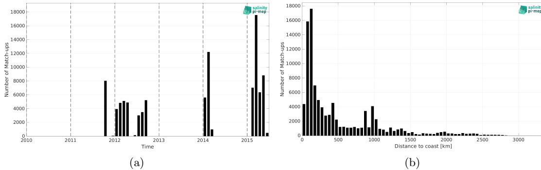
Figure 2: Number of match-ups between TSG (GOSUD-Research-vessel) and Aquarius SSS L4 OI v5 - Weekly (IPRC) SSS as a function of time (a) and as function of the distance to coast (b) over the Tropical Pacific Ocean Pi-MEP region and for the full satellite product period.
