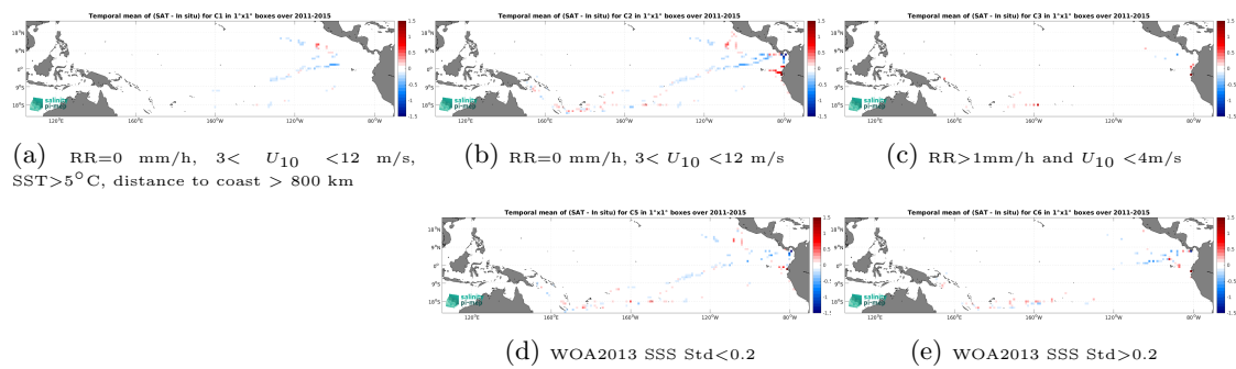
Figure 14: Temporal mean gridded over spatial boxes of size 1^\circ \times 1^\circ of \Delta\text{SSS} (Aquarius SSS L4 OI v5 - Weekly (IPRC) - TSG (GOSUD-Research-vessel)) for 5 different subdatasets corresponding to: RR=0 mm/h, 3 < U_{10} < 12 m/s, SST > 5°C, distance to coast > 800 km (a), RR=0 mm/h, 3 < U_{10} < 12 m/s (b), RR > 1mm/h and U_{10} < 4 m/s (c), WOA2013 SSS Std < 0.2 (d), WOA2013 SSS Std > 0.2 (e).
