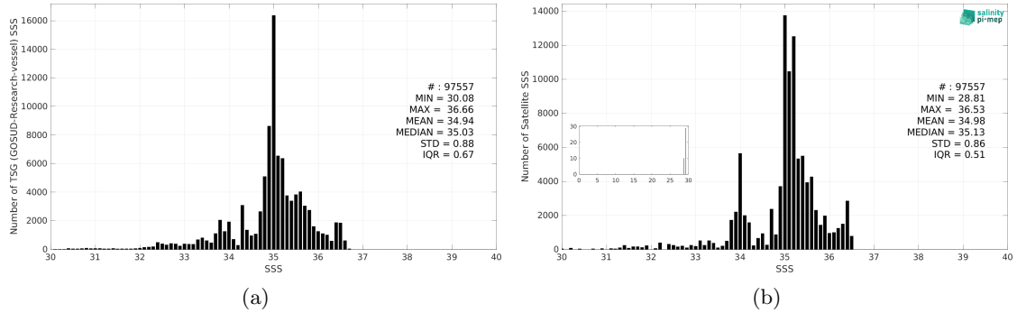
Figure 3: Histograms of SSS from TSG (GOSUD-Research-vessel) (a) and Aquarius SSS L4 OI v5 - Weekly (IPRC) (b) considering all match-up pairs per bins of 0.1 over the Tropical Pacific Ocean Pi-MEP region and for the full satellite product period.
