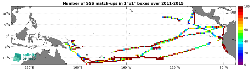
Figure 5: Number of SSS match-ups between TSG (GOSUD-Research-vessel) SSS and the Aquarius SSS L4 OI v5 - Weekly (IPRC) SSS product for the Tropical Pacific Ocean Pi-MEP region over 1^\circ \times 1^\circ boxes and for the full satellite product period.
