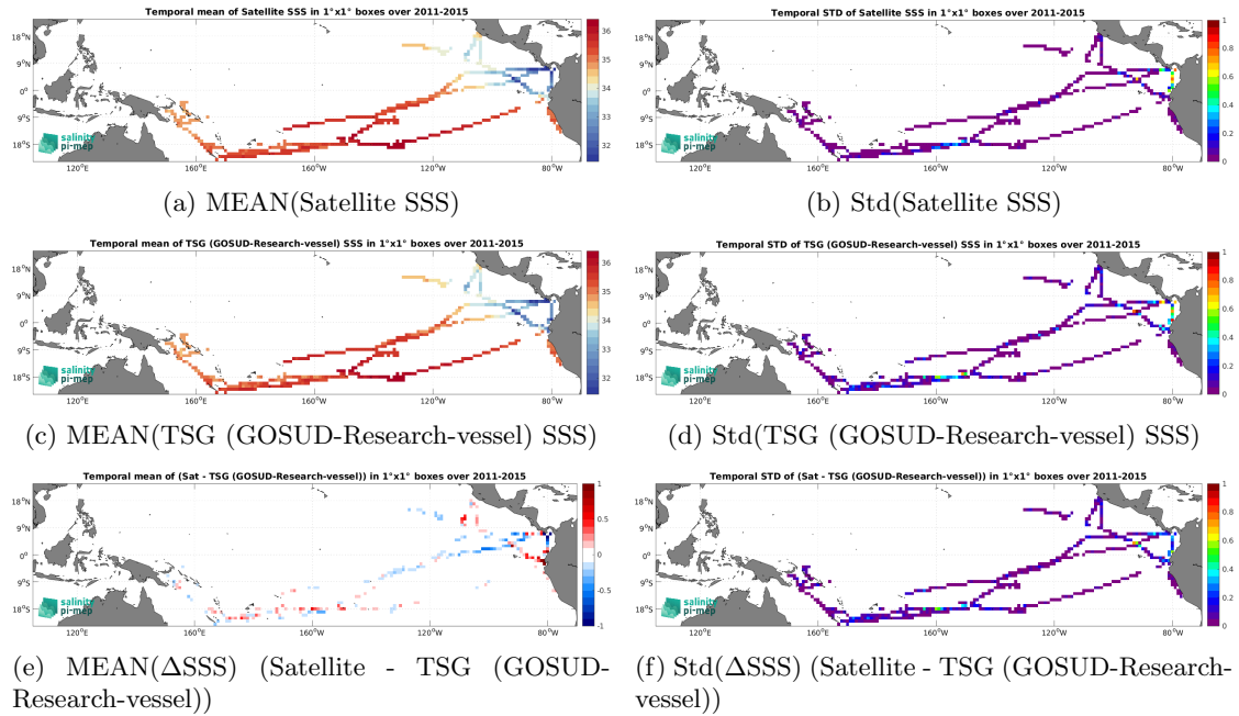
Figure 7: Temporal mean (left) and Std (right) of SSS from Aquarius SSS L4 OI v5 - Weekly (IPRC) (top), TSG (GOSUD-Research-vessel) (middle), and of \Delta SSS (Satellite - TSG (GOSUD-Research-vessel)). Only match-up pairs are used to generate these maps.
