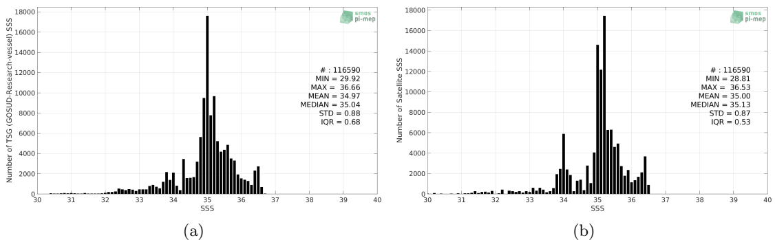
Figure 2: Histograms of SSS from TSG (GOSUD-Research-vessel) (a) and Aquarius SSS L4 OI v5 - Weekly (IPRC) (b) considering all match-up pairs per bins of 0.1 over the Tropical Pacific Ocean Pi-MEP region and for the full satellite product period.
