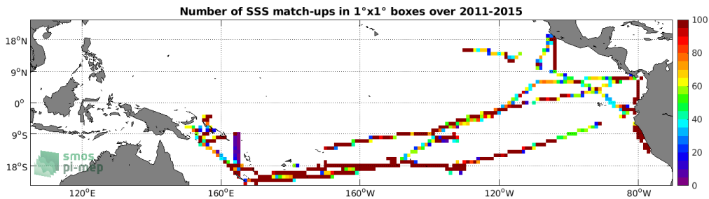
Figure 4: Number of SSS match-ups between TSG (GOSUD-Research-vessel) SSS and the Aquarius SSS L4 OI v5 - Weekly (IPRC) SSS product for the Tropical Pacific Ocean Pi-MEP region over 1^\circ \times 1^\circ boxes and for the full satellite product period.
