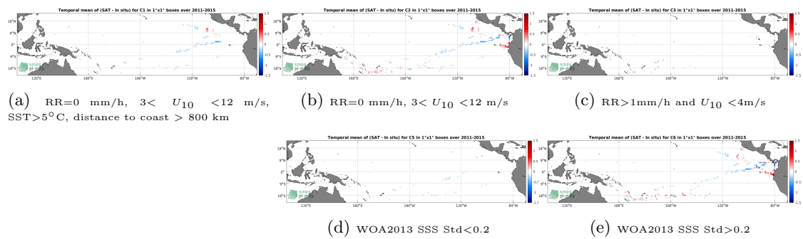
Figure 12: Temporal mean gridded over spatial boxes of size 1^\circ \times 1^\circ of \Delta\text{SSS} (Aquarius SSS L4 OI v5 - Weekly (IPRC) - TSG (GOSUD-Research-vessel)) for 5 different subdatasets corresponding to: RR=0 mm/h, 3 < U_{10} < 12 m/s, SST > 5°C, distance to coast > 800 km (a), RR=0 mm/h, 3 < U_{10} < 12 m/s (b), RR > 1mm/h and U_{10} < 4 m/s (c), WOA2013 SSS Std < 0.2 (d), WOA2013 SSS Std > 0.2 (e).
