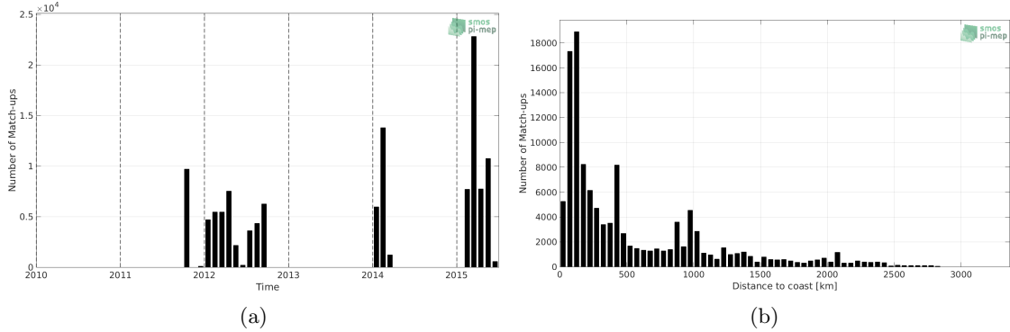
Figure 1: Number of match-ups between TSG-GOSUD-Research-vessel and Aquarius-L4-IPRC-V5-WEEKLY SSS as a function of time (a) and as function of the distance to coast (b) over the Tropical Pacific Ocean Pi-MEP region and for the full satellite product period.
