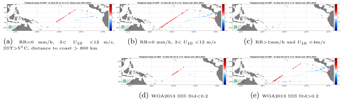
Figure 12: Temporal mean gridded over spatial boxes of size 1^\circ \times 1^\circ of \Delta SSS (Aquarius-L4-IPRC-V5-WEEKLY - TSG-GOSUD-Research-vessel) for 5 different subdatasets corresponding to: RR=0 mm/h, 3 < U_{10} < 12 m/s, SST > 5^\circ C , distance to coast > 800 km (a), RR=0 mm/h, 3 < U_{10} < 12 m/s (b), RR > 1 mm/h and U_{10} < 4 m/s (c), WOA2013 SSS Std < 0.2 (d), WOA2013 SSS Std > 0.2 (e).
