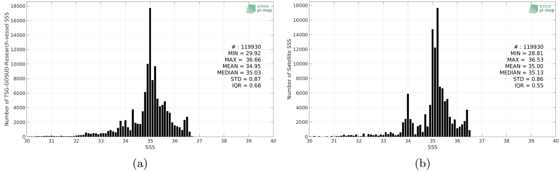
Figure 2: Histograms of SSS from TSG-GOSUD-Research-vessel (a) and Aquarius-L4-IPRC-V5-WEEKLY (b) considering all match-up pairs per bins of 0.1 over the Tropical Pacific Ocean Pi-MEP region and for the full satellite product period.
