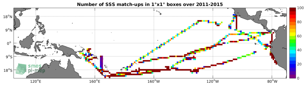
Figure 4: Number of SSS match-ups between TSG-GOSUD-Research-vessel SSS and the Aquarius-L4-IPRC-V5-WEEKLY SSS product for the Tropical Pacific Ocean Pi-MEP region over 1°x1° boxes and for the full satellite product period.
