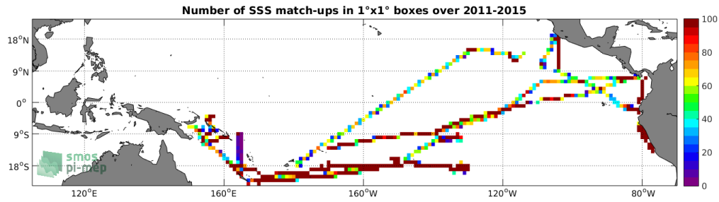
Figure 4: Number of SSS match-ups between TSG-GOSUD-Research-vessel SSS and the Aquarius-L4-IPRC-V5-WEEKLY SSS product for the Tropical Pacific Ocean Pi-MEP region over 1^\circ \times 1^\circ boxes and for the full satellite product period.
