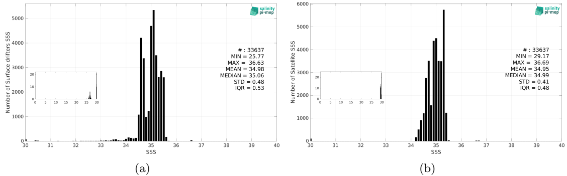
Figure 3: Histograms of SSS from Surface drifters (a) and Aquarius SSS L4 OI v5 - Weekly (IPRC) (b) considering all match-up pairs per bins of 0.1 over the Tropical Pacific Ocean Pi-MEP region and for the full satellite product period.
