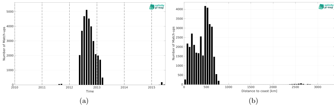
Figure 2: Number of match-ups between Surface drifters and Aquarius SSS L4 OI v5 - Weekly (IPRC) SSS as a function of time (a) and as function of the distance to coast (b) over the Tropical Pacific Ocean Pi-MEP region and for the full satellite product period.
