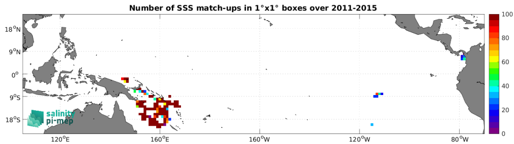
Figure 4: Number of SSS match-ups between Surface drifters SSS and the Aquarius SSS L4 OI v5 - Weekly (IPRC) SSS product for the Tropical Pacific Ocean Pi-MEP region over 1^\circ \times 1^\circ boxes and for the full satellite product period.
