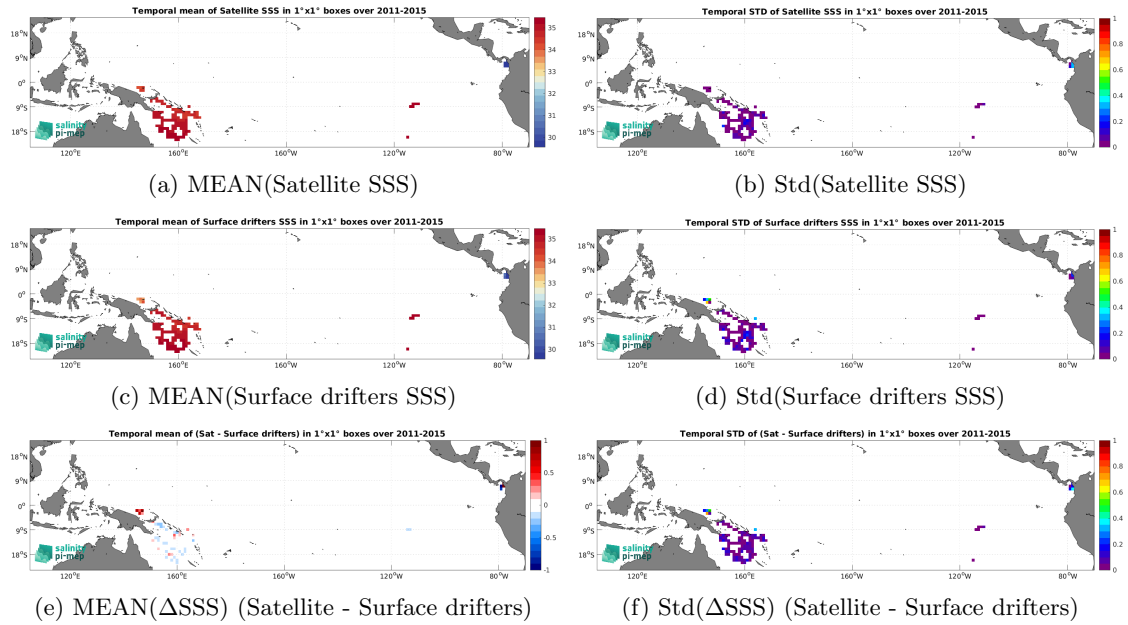
Figure 6: Temporal mean (left) and Std (right) of SSS from Aquarius SSS L4 OI v5 - Weekly (IPRC) (top), Surface drifters (middle), and of \Delta SSS (Satellite - Surface drifters). Only match-up pairs are used to generate these maps.
