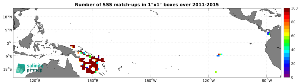
Figure 3: Number of SSS match-ups between Surface drifters SSS and the Aquarius SSS L4 OI v5 - Weekly (IPRC) SSS product for the Tropical Pacific Ocean Pi-MEP region over 1^\circ \times 1^\circ boxes and for the full satellite product period.
