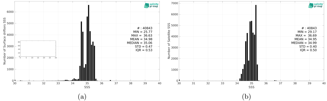
Figure 2: Histograms of SSS from Surface drifters (a) and Aquarius SSS L4 OI v5 - Weekly (IPRC) (b) considering all match-up pairs per bins of 0.1 over the Tropical Pacific Ocean Pi-MEP region and for the full satellite product period.
