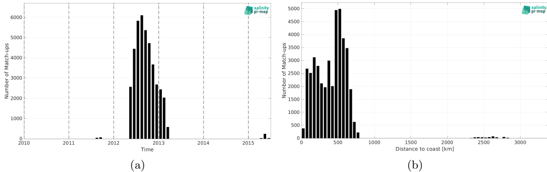
Figure 1: Number of match-ups between Surface drifters and Aquarius SSS L4 OI v5 - Weekly (IPRC) SSS as a function of time (a) and as function of the distance to coast (b) over the Tropical Pacific Ocean Pi-MEP region and for the full satellite product period.
