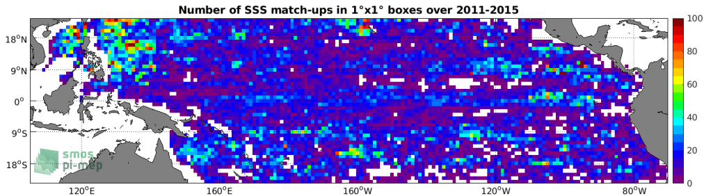
Figure 4: Number of SSS match-ups between Argo SSS and the Aquarius SSS L4 OI v5 - Weekly (IPRC) SSS product for the Tropical Pacific Ocean Pi-MEP region over 1^\circ \times 1^\circ boxes and for the full satellite product period.
