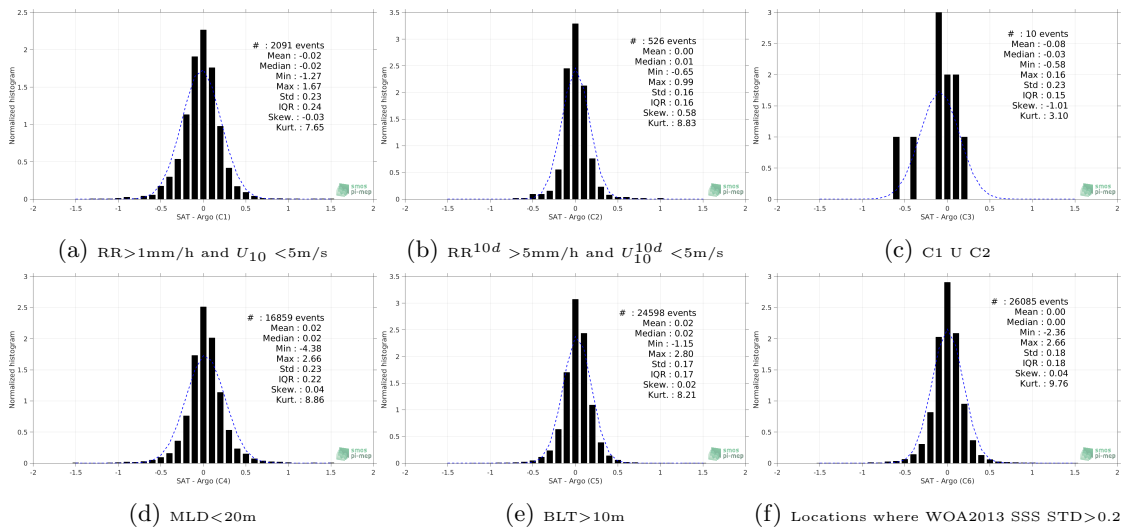
Figure 13: Normalized histogram of \Delta SSS (Aquarius-L4-IPRC-V5-WEEKLY - Argo) for 6 different subdatasets corresponding to: RR>1mm/h and U_{10} < 5m/s (a), RR^{10d} > 5mm/h and U_{10}^{10d} < 5m/s (b), C1 U C2 (c),MLD<20m (d),BLT>10m (e),Locations where WOA2013 SSS STD>0.2 (f).
