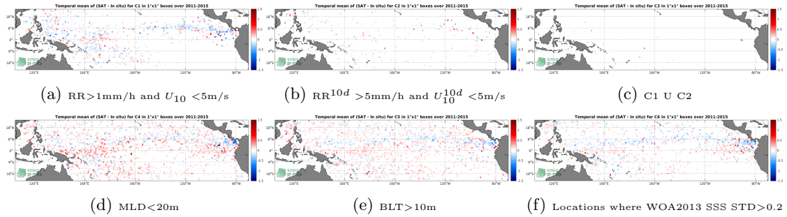
Figure 12: Temporal mean gridded over spatial boxes of size 1°x1° of \Delta SSS (Aquarius-L4-IPRC-V5-WEEKLY - Argo) for 6 different subdatasets corresponding to:RR>1mm/h and U_{10} < 5m/s (a), RR^{10d} > 5mm/h and U_{10}^{10d} < 5m/s (b), C1 U C2 (c),MLD<20m (d),BLT>10m (e),Locations where WOA2013 SSS STD>0.2 (f).
