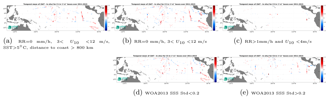
Figure 14: Temporal mean gridded over spatial boxes of size 1^\circ \times 1^\circ of \Delta SSS (Aquarius SSS L4 OI v5 - Monthly (IPRC) - TSG (SAMOS)) for 5 different subdatasets corresponding to: RR=0 mm/h, 3 < U_{10} < 12 m/s, SST > 5^\circ\text{C} , distance to coast > 800 km (a), RR=0 mm/h, 3 < U_{10} < 12 m/s (b), RR > 1 mm/h and U_{10} < 4 m/s (c), WOA2013 SSS Std < 0.2 (d), WOA2013 SSS Std > 0.2 (e).
