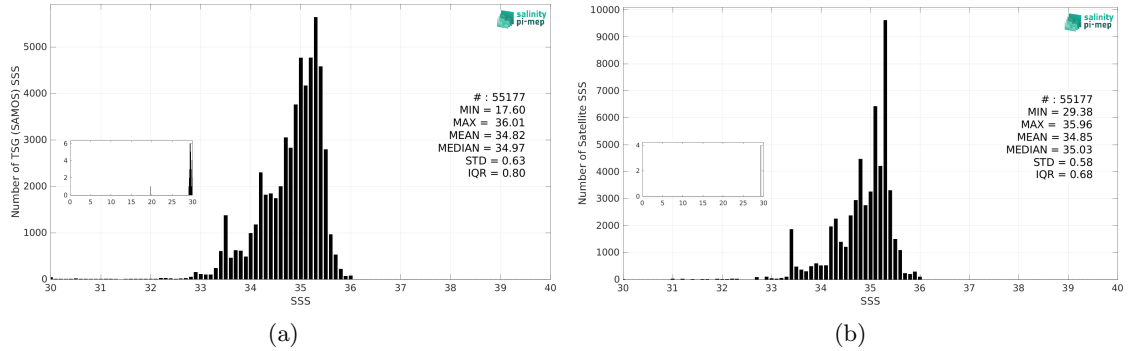
Figure 3: Histograms of SSS from TSG (SAMOS) (a) and Aquarius SSS L4 OI v5 - Monthly (IPRC) (b) considering all match-up pairs per bins of 0.1 over the Tropical Pacific Ocean Pi-MEP region and for the full satellite product period.
