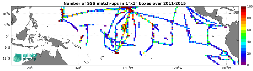
Figure 5: Number of SSS match-ups between TSG (SAMOS) SSS and the Aquarius SSS L4 OI v5 - Monthly (IPRC) SSS product for the Tropical Pacific Ocean Pi-MEP region over 1^\circ \times 1^\circ boxes and for the full satellite product period.
