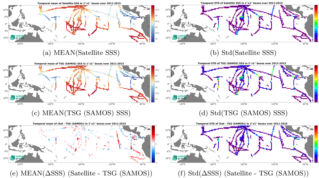
Figure 7: Temporal mean (left) and Std (right) of SSS from Aquarius SSS L4 OI v5 - Monthly (IPRC) (top), TSG (SAMOS) (middle), and of \Delta SSS (Satellite - TSG (SAMOS)). Only match-up pairs are used to generate these maps.
