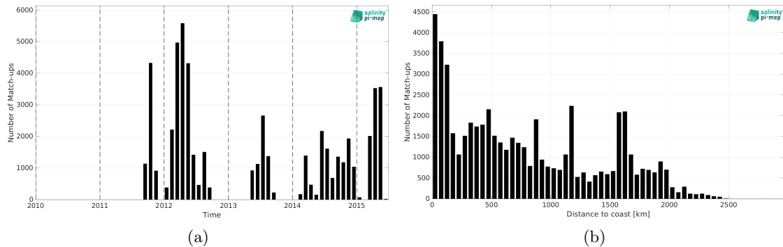
Figure 2: Number of match-ups between TSG (SAMOS) and Aquarius SSS L4 OI v5 - Monthly (IPRC) SSS as a function of time (a) and as function of the distance to coast (b) over the Tropical Pacific Ocean Pi-MEP region and for the full satellite product period.
