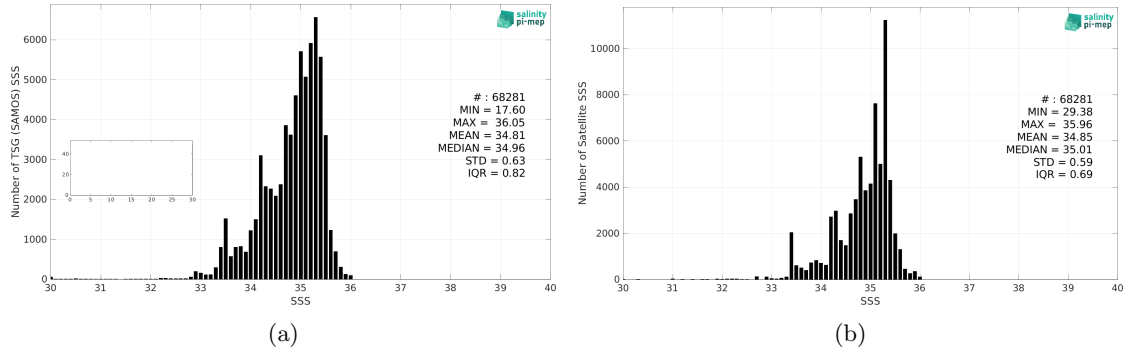
Figure 2: Histograms of SSS from TSG (SAMOS) (a) and Aquarius SSS L4 OI v5 - Monthly (IPRC) (b) considering all match-up pairs per bins of 0.1 over the Tropical Pacific Ocean Pi-MEP region and for the full satellite product period.
