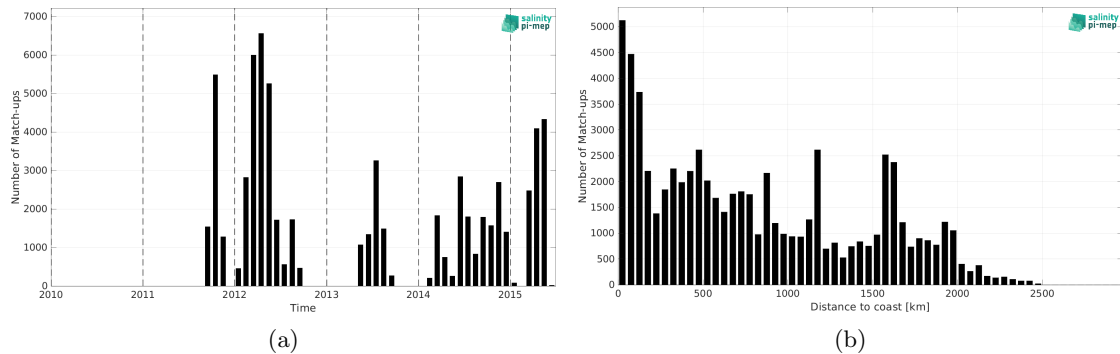
Figure 1: Number of match-ups between TSG (SAMOS) and Aquarius SSS L4 OI v5 - Monthly (IPRC) SSS as a function of time (a) and as function of the distance to coast (b) over the Tropical Pacific Ocean Pi-MEP region and for the full satellite product period.
