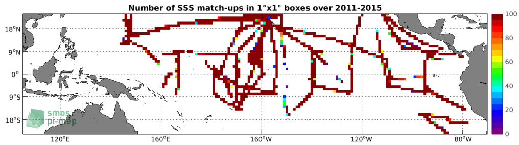
Figure 4: Number of SSS match-ups between TSG (SAMOS) SSS and the Aquarius SSS L4 OI v5 - Monthly (IPRC) SSS product for the Tropical Pacific Ocean Pi-MEP region over 1°x1° boxes and for the full satellite product period.
