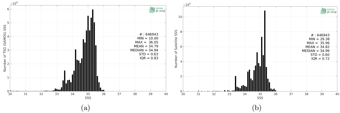
Figure 2: Histograms of SSS from TSG (SAMOS) (a) and Aquarius SSS L4 OI v5 - Monthly (IPRC) (b) considering all match-up pairs per bins of 0.1 over the Tropical Pacific Ocean Pi-MEP region and for the full satellite product period.
