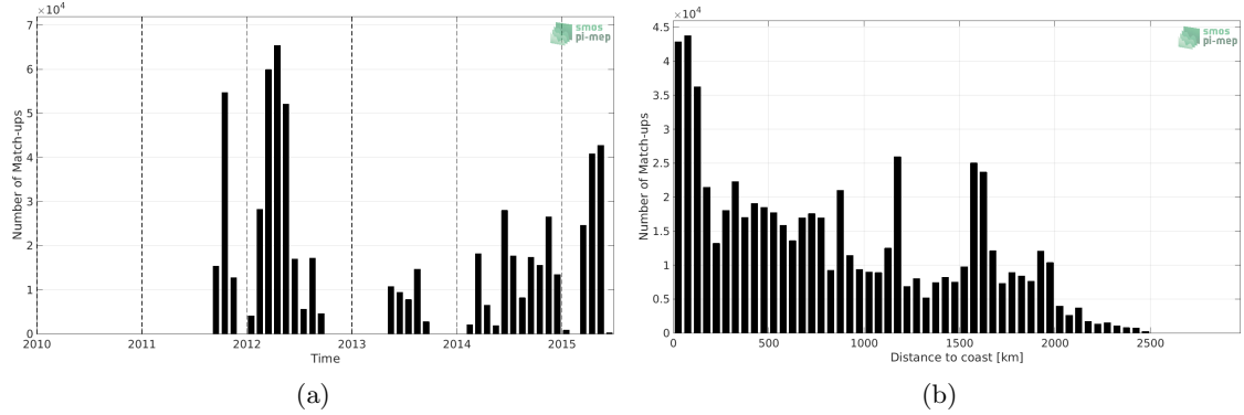
Figure 1: Number of match-ups between TSG (SAMOS) and Aquarius SSS L4 OI v5 - Monthly (IPRC) SSS as a function of time (a) and as function of the distance to coast (b) over the Tropical Pacific Ocean Pi-MEP region and for the full satellite product period.
