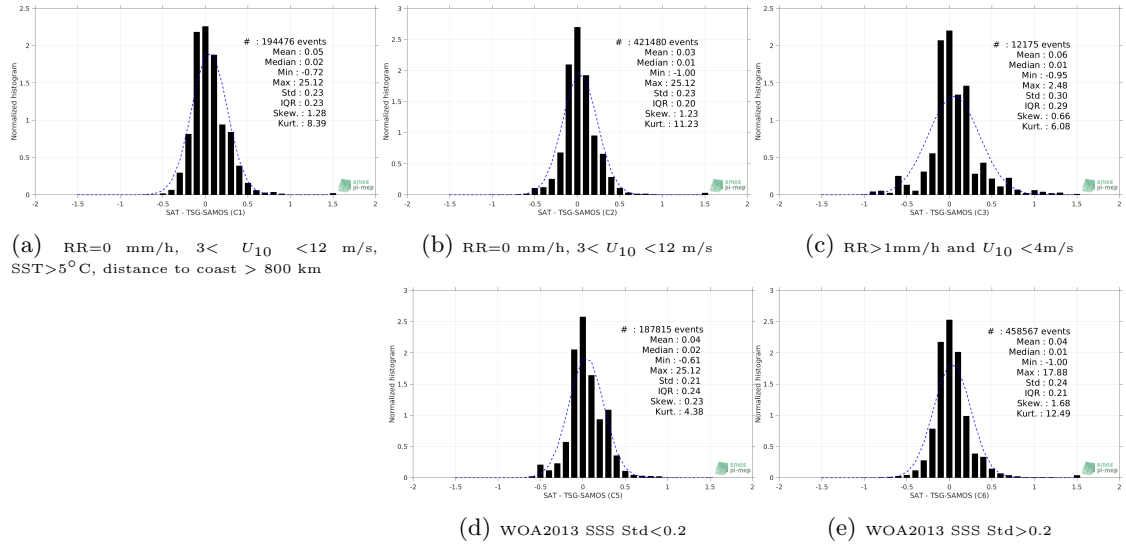
Figure 13: Normalized histogram of \Delta SSS (Aquarius-L4-IPRC-V5-MONTHLY - TSG-SAMOS) for 5 different subdatasets corresponding to: RR=0 mm/h, 3 < U_{10} < 12 m/s, SST >5^\circ C, distance to coast > 800 km (a), RR=0 mm/h, 3 < U_{10} < 12 m/s (b), RR >1 mm/h and U_{10} < 4 m/s (c), WOA2013 SSS Std <0.2 (d), WOA2013 SSS Std >0.2 (e).
