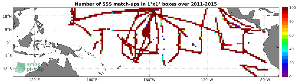
Figure 4: Number of SSS match-ups between TSG-SAMOS SSS and the Aquarius-L4-IPRC-V5-MONTHLY SSS product for the Tropical Pacific Ocean Pi-MEP region over 1°x1° boxes and for the full satellite product period.
