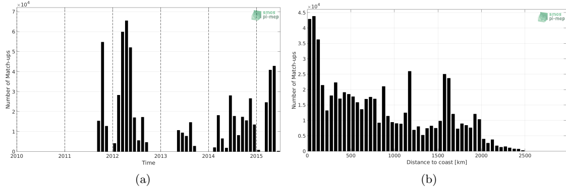
Figure 1: Number of match-ups between TSG-SAMOS and Aquarius-L4-IPRC-V5-MONTHLY SSS as a function of time (a) and as function of the distance to coast (b) over the Tropical Pacific Ocean Pi-MEP region and for the full satellite product period.
