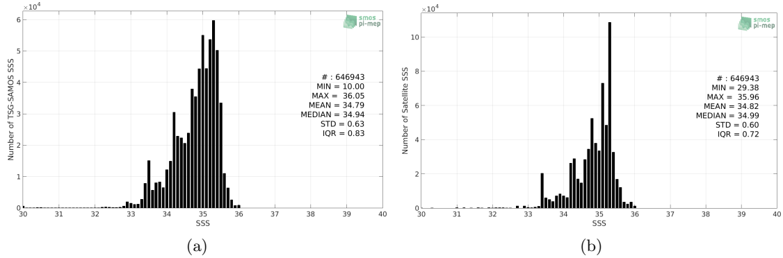
Figure 2: Histograms of SSS from TSG-SAMOS (a) and Aquarius-L4-IPRC-V5-MONTHLY (b) considering all match-up pairs per bins of 0.1 over the Tropical Pacific Ocean Pi-MEP region and for the full satellite product period.
