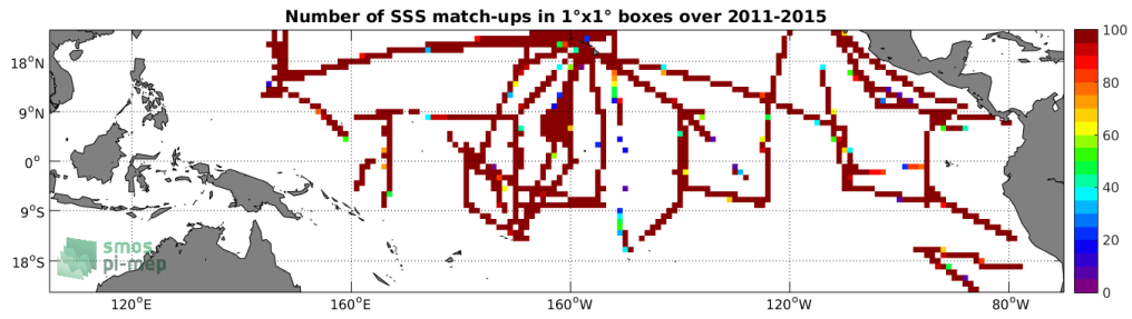
Figure 4: Number of SSS match-ups between TSG-SAMOS SSS and the Aquarius-L4-IPRC-V5-MONTHLY SSS product for the Tropical Pacific Ocean Pi-MEP region over 1^\circ \times 1^\circ boxes and for the full satellite product period.
