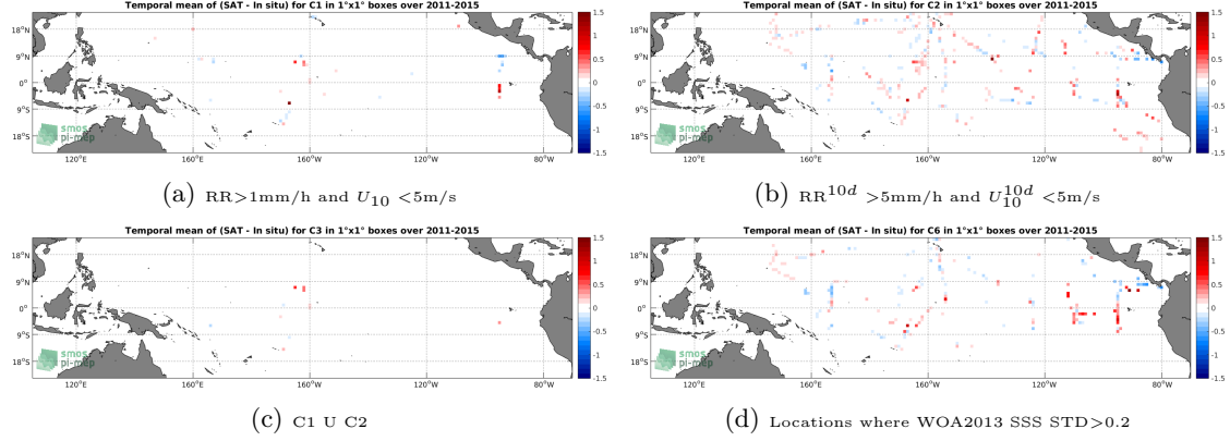
Figure 12: Temporal mean gridded over spatial boxes of size 1^\circ \times 1^\circ of \Delta SSS (Aquarius-L4-IPRC-V5-MONTHLY - TSG-SAMOS) for 4 different subdatasets corresponding to: RR > 1\text{mm/h} and U_{10} < 5\text{m/s} (a), RR^{10d} > 5\text{mm/h} and U_{10}^{10d} < 5\text{m/s} (b), C1 U C2 (c), Locations where WOA2013 SSS STD > 0.2 (d).
