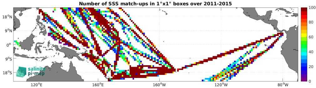
Figure 4: Number of SSS match-ups between TSG (LEGOS-DM) SSS and the Aquarius SSS L4 OI v5 - Monthly (IPRC) SSS product for the Tropical Pacific Ocean Pi-MEP region over 1^\circ \times 1^\circ boxes and for the full satellite product period.
