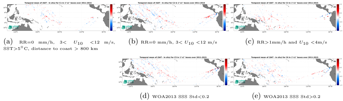
Figure 12: Temporal mean gridded over spatial boxes of size 1^\circ \times 1^\circ of \Delta\text{SSS} (Aquarius SSS L4 OI v5 - Monthly (IPRC) - TSG (LEGOS-DM)) for 5 different subdatasets corresponding to:RR=0 mm/h, 3 < U_{10} < 12 m/s, SST > 5^\circ\text{C} , distance to coast > 800 km (a), RR=0 mm/h, 3 < U_{10} < 12 m/s (b), RR > 1 mm/h and U_{10} < 4 m/s (c), WOA2013 SSS Std < 0.2 (d), WOA2013 SSS Std > 0.2 (e).
