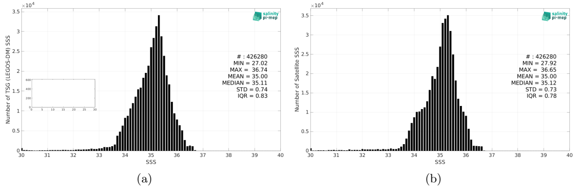
Figure 2: Histograms of SSS from TSG (LEGOS-DM) (a) and Aquarius SSS L4 OI v5 - Monthly (IPRC) (b) considering all match-up pairs per bins of 0.1 over the Tropical Pacific Ocean Pi-MEP region and for the full satellite product period.
