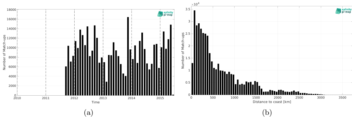
Figure 1: Number of match-ups between TSG (LEGOS-DM) and Aquarius SSS L4 OI v5 - Monthly (IPRC) SSS as a function of time (a) and as function of the distance to coast (b) over the Tropical Pacific Ocean Pi-MEP region and for the full satellite product period.
