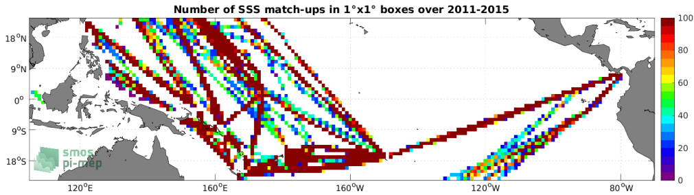
Figure 4: Number of SSS match-ups between TSG (LEGOS-DM) SSS and the Aquarius SSS L4 OI v5 - Monthly (IPRC) SSS product for the Tropical Pacific Ocean Pi-MEP region over 1^\circ \times 1^\circ boxes and for the full satellite product period.
