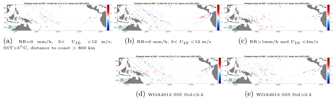
Figure 12: Temporal mean gridded over spatial boxes of size 1^\circ \times 1^\circ of \Delta SSS (Aquarius SSS L4 OI v5 - Monthly (IPRC) - TSG (LEGOS-DM)) for 5 different subdatasets corresponding to:RR=0 mm/h, 3 < U_{10} < 12 m/s, SST >5^\circ C, distance to coast > 800 km (a), RR=0 mm/h, 3 < U_{10} < 12 m/s (b), RR >1 mm/h and U_{10} < 4 m/s (c), WOA2013 SSS Std <0.2 (d), WOA2013 SSS Std >0.2 (e).
