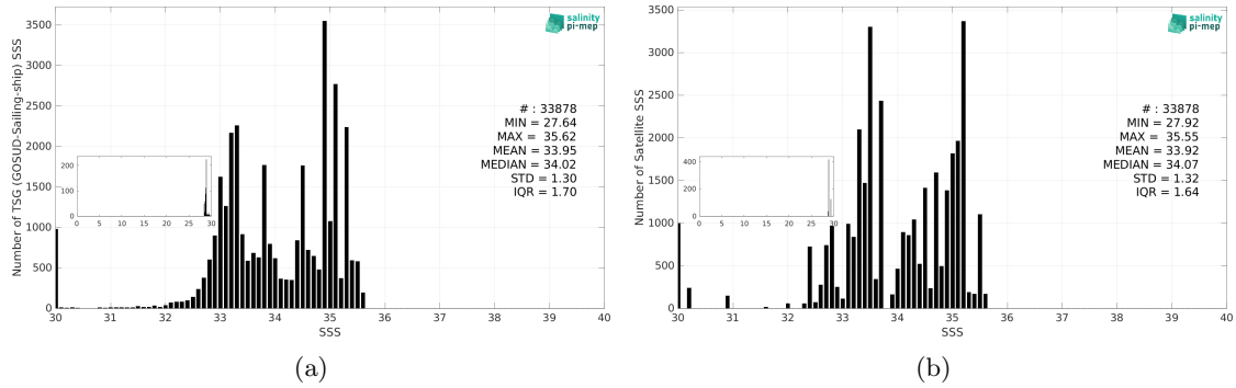
Figure 3: Histograms of SSS from TSG (GOSUD-Sailing-ship) (a) and Aquarius SSS L4 OI v5 - Monthly (IPRC) (b) considering all match-up pairs per bins of 0.1 over the Tropical Pacific Ocean Pi-MEP region and for the full satellite product period.
