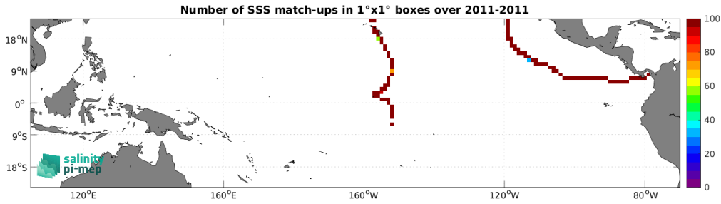
Figure 5: Number of SSS match-ups between TSG (GOSUD-Sailing-ship) SSS and the Aquarius SSS L4 OI v5 - Monthly (IPRC) SSS product for the Tropical Pacific Ocean Pi-MEP region over 1^\circ \times 1^\circ boxes and for the full satellite product period.
