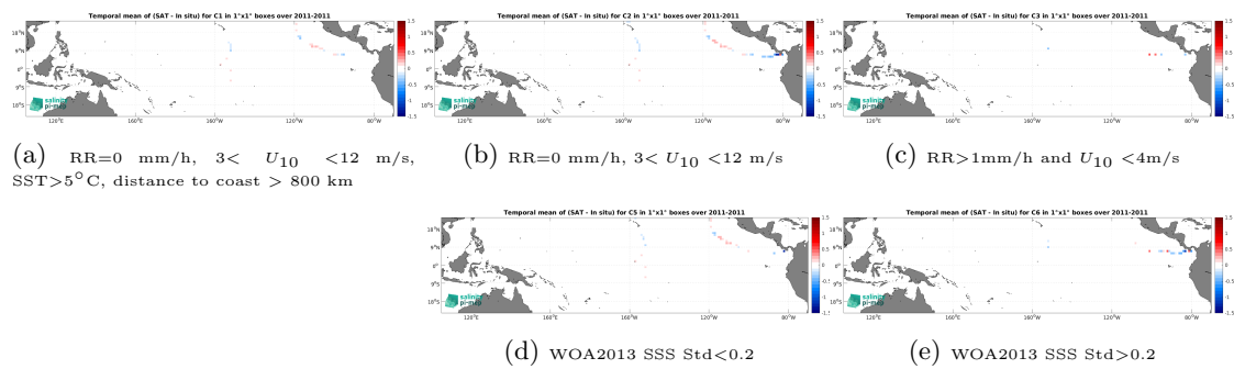
Figure 14: Temporal mean gridded over spatial boxes of size 1^\circ \times 1^\circ of \Delta SSS (Aquarius SSS L4 OI v5 - Monthly (IPRC) - TSG (GOSUD-Sailing-ship)) for 5 different subdatasets corresponding to:RR=0 mm/h, 3 < U_{10} < 12 m/s, SST >5^\circ\text{C} , distance to coast > 800 km (a), RR=0 mm/h, 3 < U_{10} < 12 m/s (b), RR >1 mm/h and U_{10} < 4 m/s (c), WOA2013 SSS Std <0.2 (d), WOA2013 SSS Std >0.2 (e).
