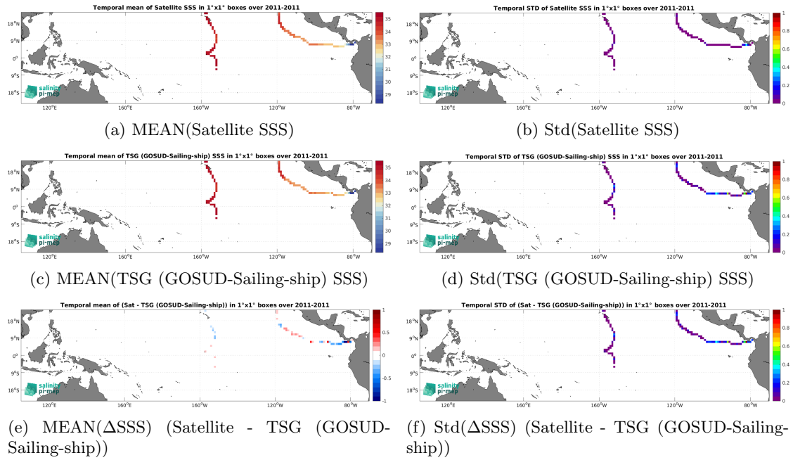
Figure 7: Temporal mean (left) and Std (right) of SSS from Aquarius SSS L4 OI v5 - Monthly (IPRC) (top), TSG (GOSUD-Sailing-ship) (middle), and of \Delta SSS (Satellite - TSG (GOSUD-Sailing-ship)). Only match-up pairs are used to generate these maps.
