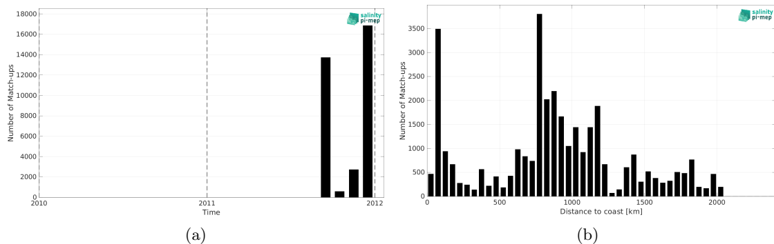
Figure 2: Number of match-ups between TSG (GOSUD-Sailing-ship) and Aquarius SSS L4 OI v5 - Monthly (IPRC) SSS as a function of time (a) and as function of the distance to coast (b) over the Tropical Pacific Ocean Pi-MEP region and for the full satellite product period.
