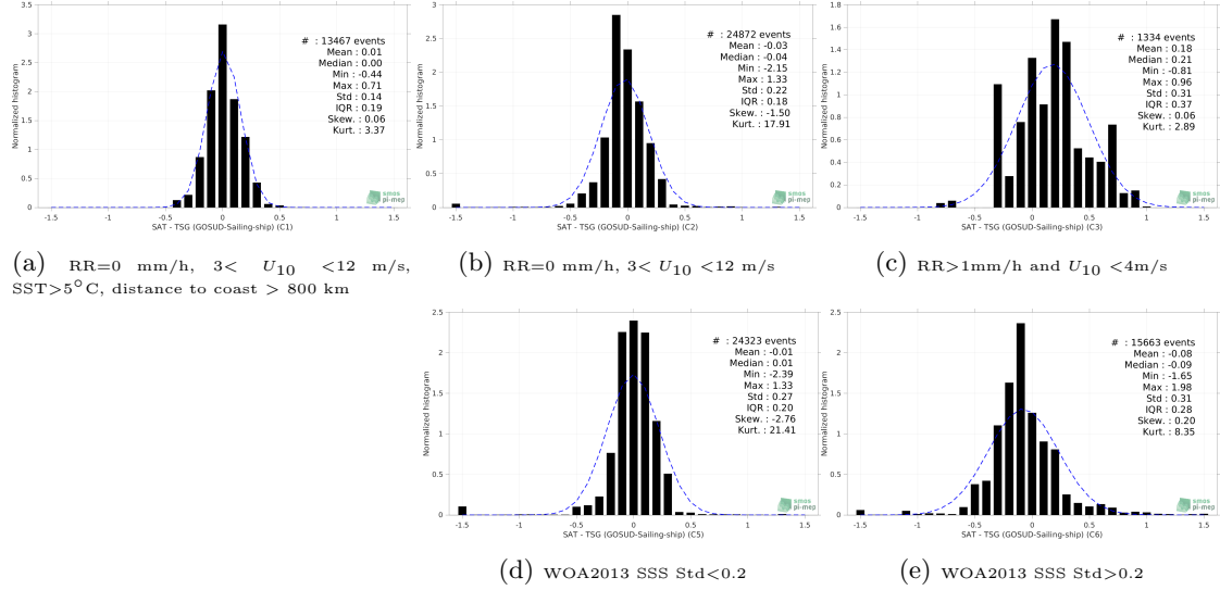
Figure 13: Normalized histogram of \Delta SSS (Aquarius SSS L4 OI v5 - Monthly (IPRC) - TSG (GOSUD-Sailing-ship)) for 5 different subdatasets corresponding to: RR=0 mm/h, 3 < U_{10} < 12 m/s, SST>5°C, distance to coast > 800 km (a), RR=0 mm/h, 3 < U_{10} < 12 m/s (b), RR>1mm/h and U_{10} < 4 m/s (c), WOA2013 SSS Std<0.2 (d), WOA2013 SSS Std>0.2 (e).
