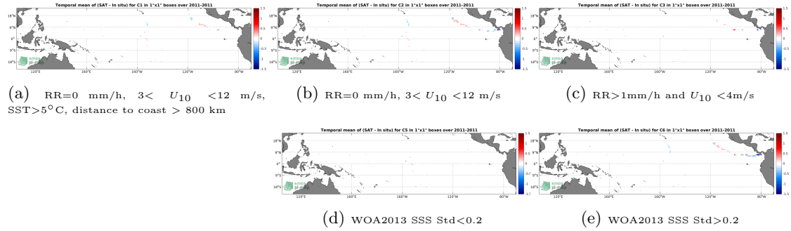
Figure 12: Temporal mean gridded over spatial boxes of size 1^\circ \times 1^\circ of \Delta SSS (Aquarius SSS L4 OI v5 - Monthly (IPRC) - TSG (GOSUD-Sailing-ship)) for 5 different subdatasets corresponding to: RR=0 mm/h, 3 < U_{10} < 12 m/s, SST > 5^\circ C , distance to coast > 800 km (a), RR=0 mm/h, 3 < U_{10} < 12 m/s (b), RR > 1 mm/h and U_{10} < 4 m/s (c), WOA2013 SSS Std < 0.2 (d), WOA2013 SSS Std > 0.2 (e).
