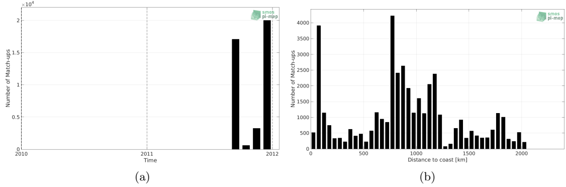
Figure 1: Number of match-ups between TSG (GOSUD-Sailing-ship) and Aquarius SSS L4 OI v5 - Monthly (IPRC) SSS as a function of time (a) and as function of the distance to coast (b) over the Tropical Pacific Ocean Pi-MEP region and for the full satellite product period.
