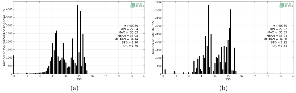
Figure 2: Histograms of SSS from TSG (GOSUD-Sailing-ship) (a) and Aquarius SSS L4 OI v5 - Monthly (IPRC) (b) considering all match-up pairs per bins of 0.1 over the Tropical Pacific Ocean Pi-MEP region and for the full satellite product period.
