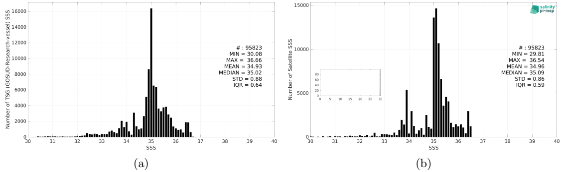
Figure 3: Histograms of SSS from TSG (GOSUD-Research-vessel) (a) and Aquarius SSS L4 OI v5 - Monthly (IPRC) (b) considering all match-up pairs per bins of 0.1 over the Tropical Pacific Ocean Pi-MEP region and for the full satellite product period.
