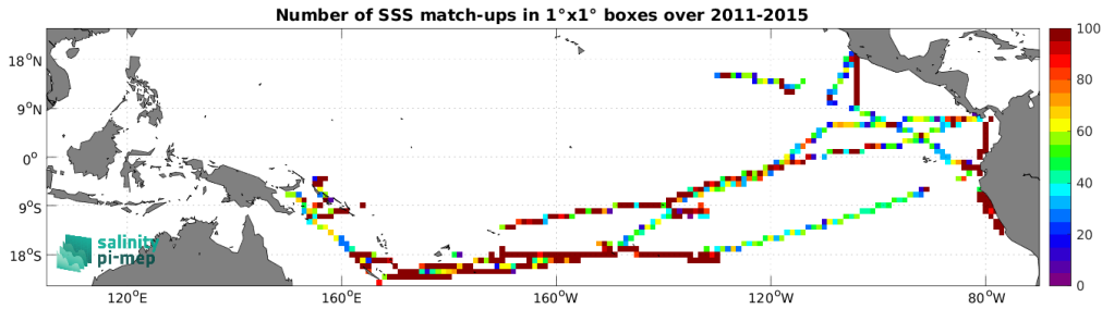
Figure 5: Number of SSS match-ups between TSG (GOSUD-Research-vessel) SSS and the Aquarius SSS L4 OI v5 - Monthly (IPRC) SSS product for the Tropical Pacific Ocean Pi-MEP region over 1^\circ \times 1^\circ boxes and for the full satellite product period.
