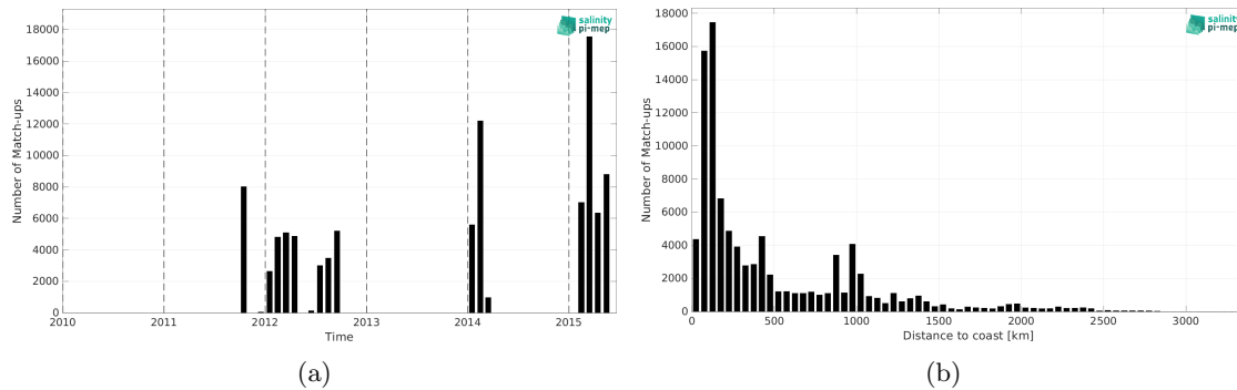
Figure 2: Number of match-ups between TSG (GOSUD-Research-vessel) and Aquarius SSS L4 OI v5 - Monthly (IPRC) SSS as a function of time (a) and as function of the distance to coast (b) over the Tropical Pacific Ocean Pi-MEP region and for the full satellite product period.
