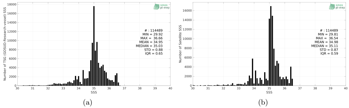
Figure 2: Histograms of SSS from TSG (GOSUD-Research-vessel) (a) and Aquarius SSS L4 OI v5 - Monthly (IPRC) (b) considering all match-up pairs per bins of 0.1 over the Tropical Pacific Ocean Pi-MEP region and for the full satellite product period.
