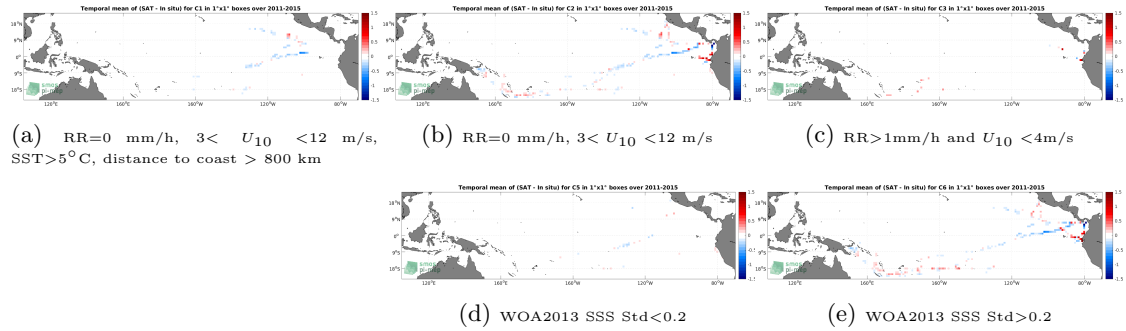
Figure 12: Temporal mean gridded over spatial boxes of size 1^{\circ}\times 1^{\circ} of \Delta SSS (Aquarius SSS L4 OI v5 - Monthly (IPRC) - TSG (GOSUD-Research-vessel)) for 5 different subdatasets corresponding to:RR=0 mm/h, 3 < U_{10} < 12 m/s, SST >5^{\circ}\text{C} , distance to coast > 800 km (a), RR=0 mm/h, 3 < U_{10} < 12 m/s (b), RR >1 mm/h and U_{10} < 4 m/s (c), WOA2013 SSS Std <0.2 (d), WOA2013 SSS Std >0.2 (e).
