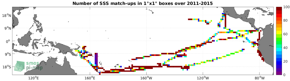
Figure 4: Number of SSS match-ups between TSG (GOSUD-Research-vessel) SSS and the Aquarius SSS L4 OI v5 - Monthly (IPRC) SSS product for the Tropical Pacific Ocean Pi-MEP region over 1^\circ \times 1^\circ boxes and for the full satellite product period.
