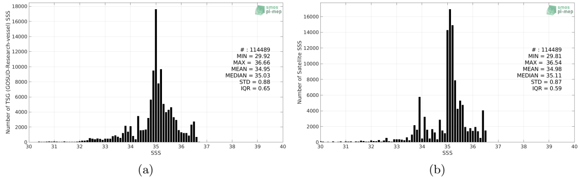
Figure 2: Histograms of SSS from TSG (GOSUD-Research-vessel) (a) and Aquarius SSS L4 OI v5 - Monthly (IPRC) (b) considering all match-up pairs per bins of 0.1 over the Tropical Pacific Ocean Pi-MEP region and for the full satellite product period.
