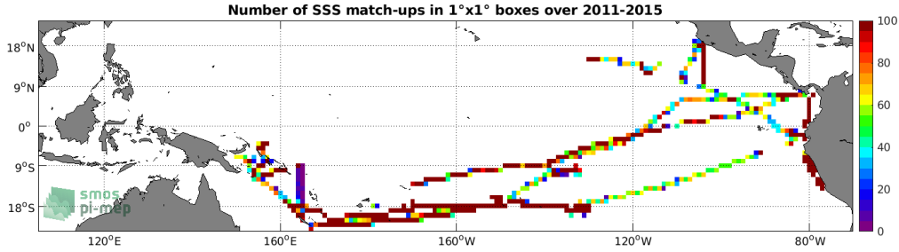
Figure 4: Number of SSS match-ups between TSG (GOSUD-Research-vessel) SSS and the Aquarius SSS L4 OI v5 - Monthly (IPRC) SSS product for the Tropical Pacific Ocean Pi-MEP region over 1^\circ \times 1^\circ boxes and for the full satellite product period.
