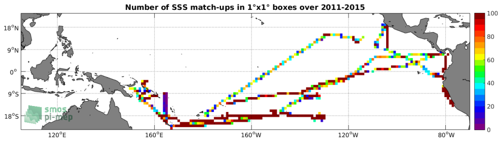
Figure 4: Number of SSS match-ups between TSG-GOSUD-Research-vessel SSS and the Aquarius-L4-IPRC-V5-MONTHLY SSS product for the Tropical Pacific Ocean Pi-MEP region over 1^\circ \times 1^\circ boxes and for the full satellite product period.
