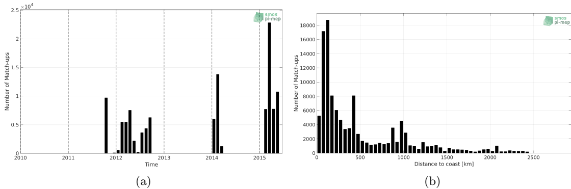
Figure 1: Number of match-ups between TSG-GOSUD-Research-vessel and Aquarius-L4-IPRC-V5-MONTHLY SSS as a function of time (a) and as function of the distance to coast (b) over the Tropical Pacific Ocean Pi-MEP region and for the full satellite product period.
