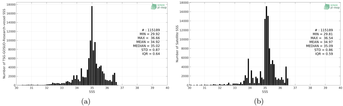
Figure 2: Histograms of SSS from TSG-GOSUD-Research-vessel (a) and Aquarius-L4-IPRC-V5-MONTHLY (b) considering all match-up pairs per bins of 0.1 over the Tropical Pacific Ocean Pi-MEP region and for the full satellite product period.
